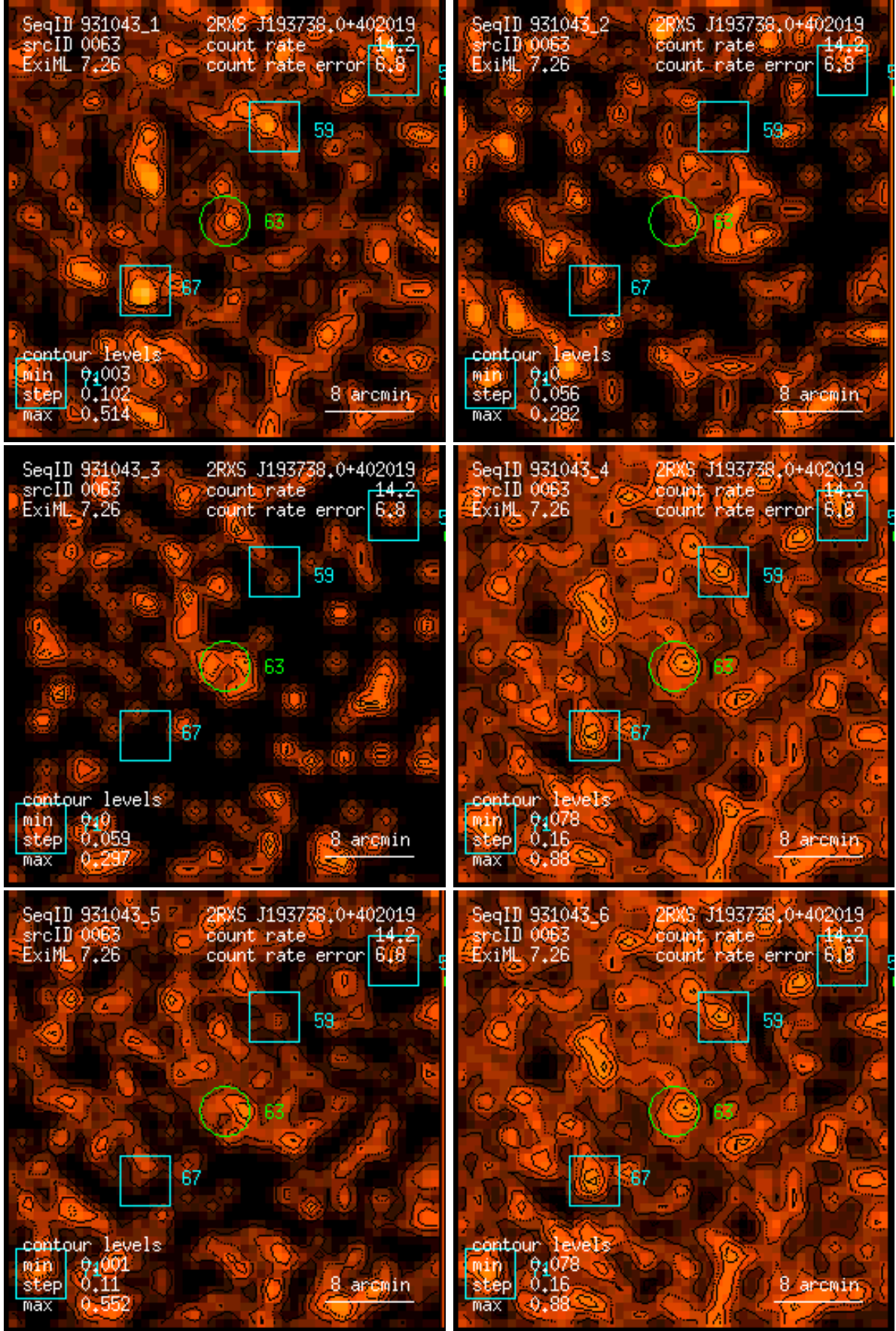
Figure 63: RASS 931043: detection 0063: band rate images, Gaussian filter: (1) PSPC channels 11 – 41, (2) 52 – 90, (3) 91 – 201, (4) 11 – 235, (5) 52 – 201, (6) 11 – 201. Broad band rates in counts/ks. Band rate contour levels in counts/ks/arcmin 2 .
