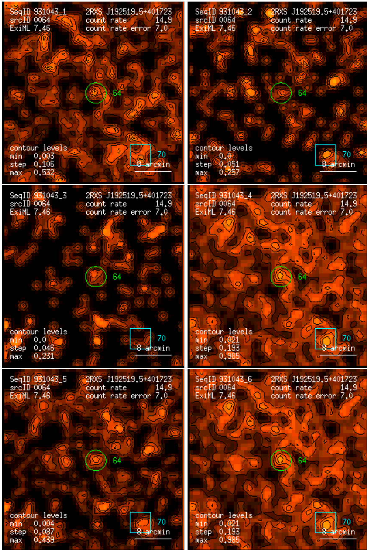
Figure 64: RASS 931043: detection 0064: band rate images, Gaussian filter: (1) PSPC channels 11 – 41, (2) 52 – 90, (3) 91 – 201, (4) 11 – 235, (5) 52 – 201, (6) 11 – 201. Broad band rates in counts/ks. Band rate contour levels in counts/ks/arcmin 2 .
