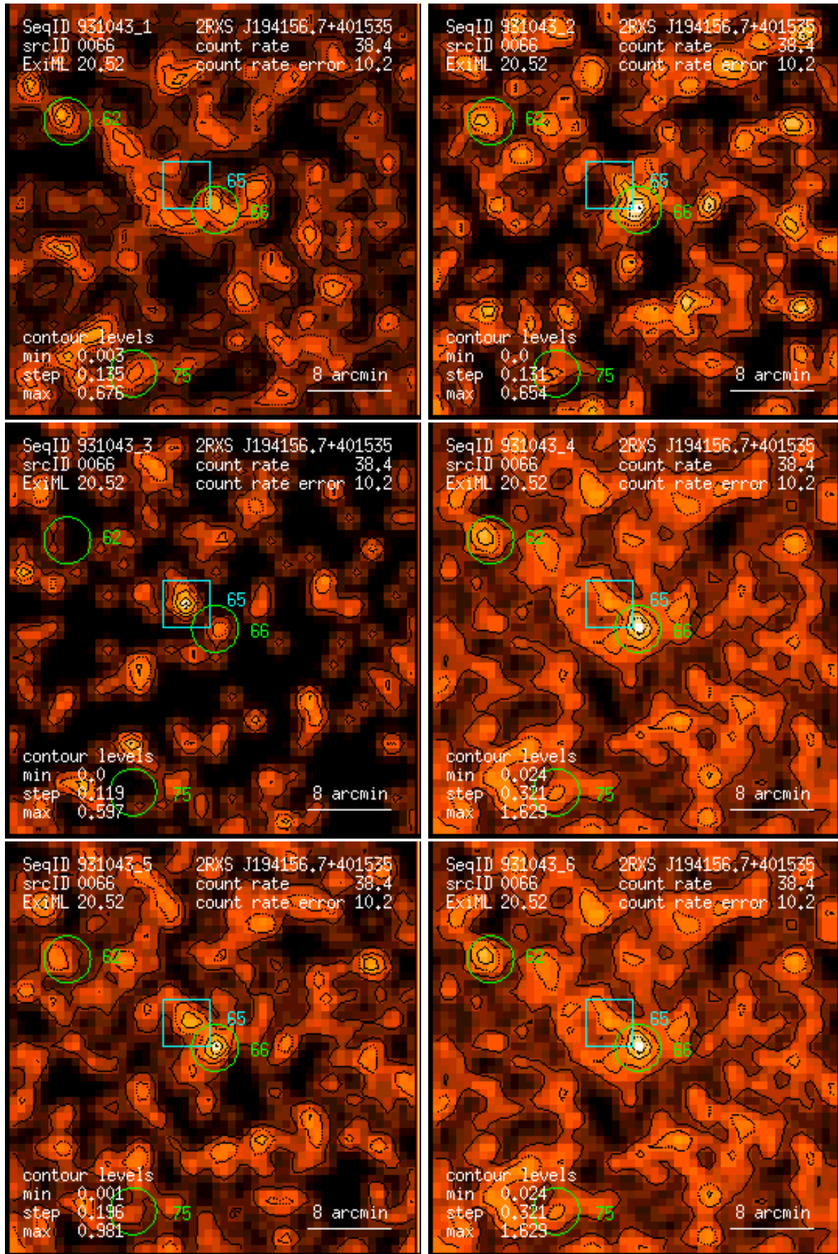
Figure 66: RASS 931043: detection 0066: band rate images, Gaussian filter: (1) PSPC channels 11 – 41, (2) 52 – 90, (3) 91 – 201, (4) 11 – 235, (5) 52 – 201, (6) 11 – 201. Broad band rates in counts/ks. Band rate contour levels in counts/ks/arcmin 2 .
