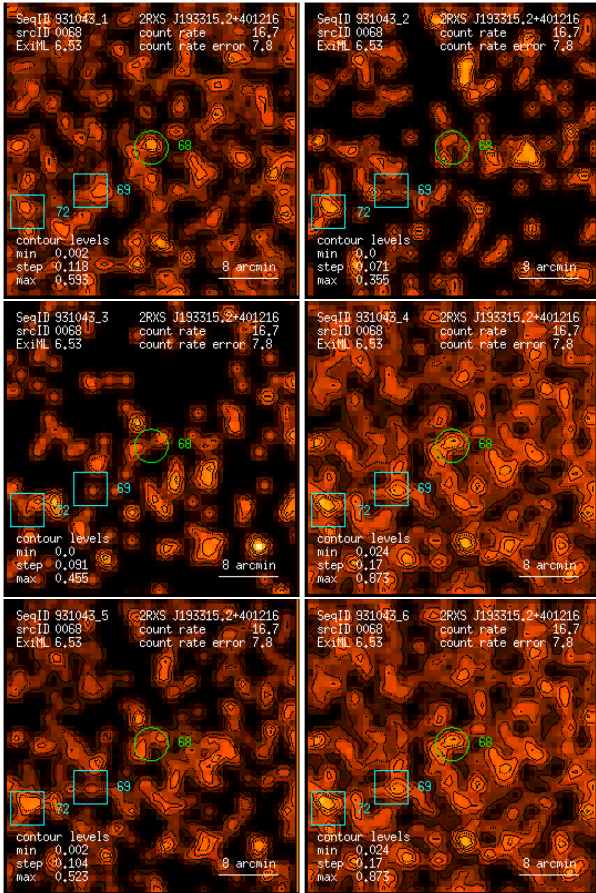
Figure 68: RASS 931043: detection 0068: band rate images, Gaussian filter: (1) PSPC channels 11 – 41, (2) 52 – 90, (3) 91 – 201, (4) 11 – 235, (5) 52 – 201, (6) 11 – 201. Broad band rates in counts/ks. Band rate contour levels in counts/ks/arcmin 2 .
