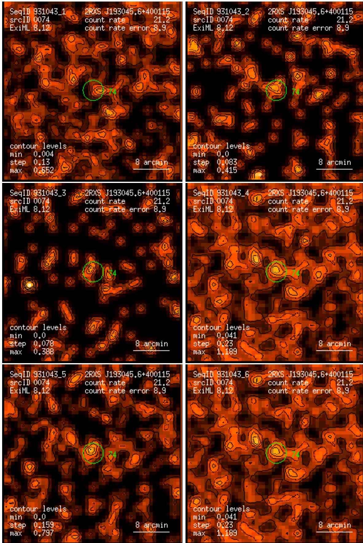
Figure 74: RASS 931043: detection 0074: band rate images, Gaussian filter: (1) PSPC channels 11 – 41, (2) 52 – 90, (3) 91 – 201, (4) 11 – 235, (5) 52 – 201, (6) 11 – 201. Broad band rates in counts/ks. Band rate contour levels in counts/ks/arcmin 2 .
