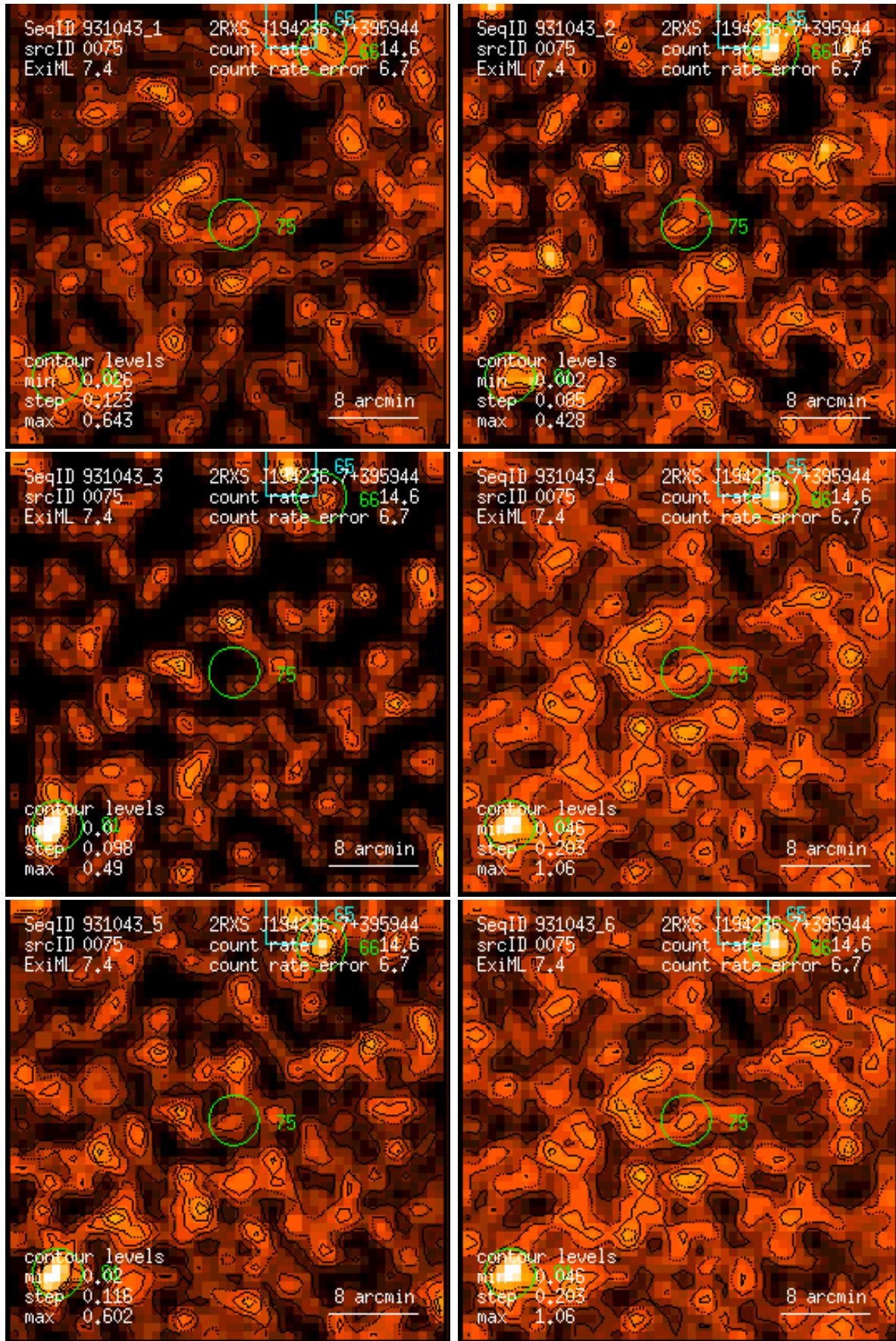
Figure 75: RASS 931043: detection 0075: band rate images, Gaussian filter: (1) PSPC channels 11 – 41, (2) 52 – 90, (3) 91 – 201, (4) 11 – 235, (5) 52 – 201, (6) 11 – 201. Broad band rates in counts/ks. Band rate contour levels in counts/ks/arcmin 2 .
