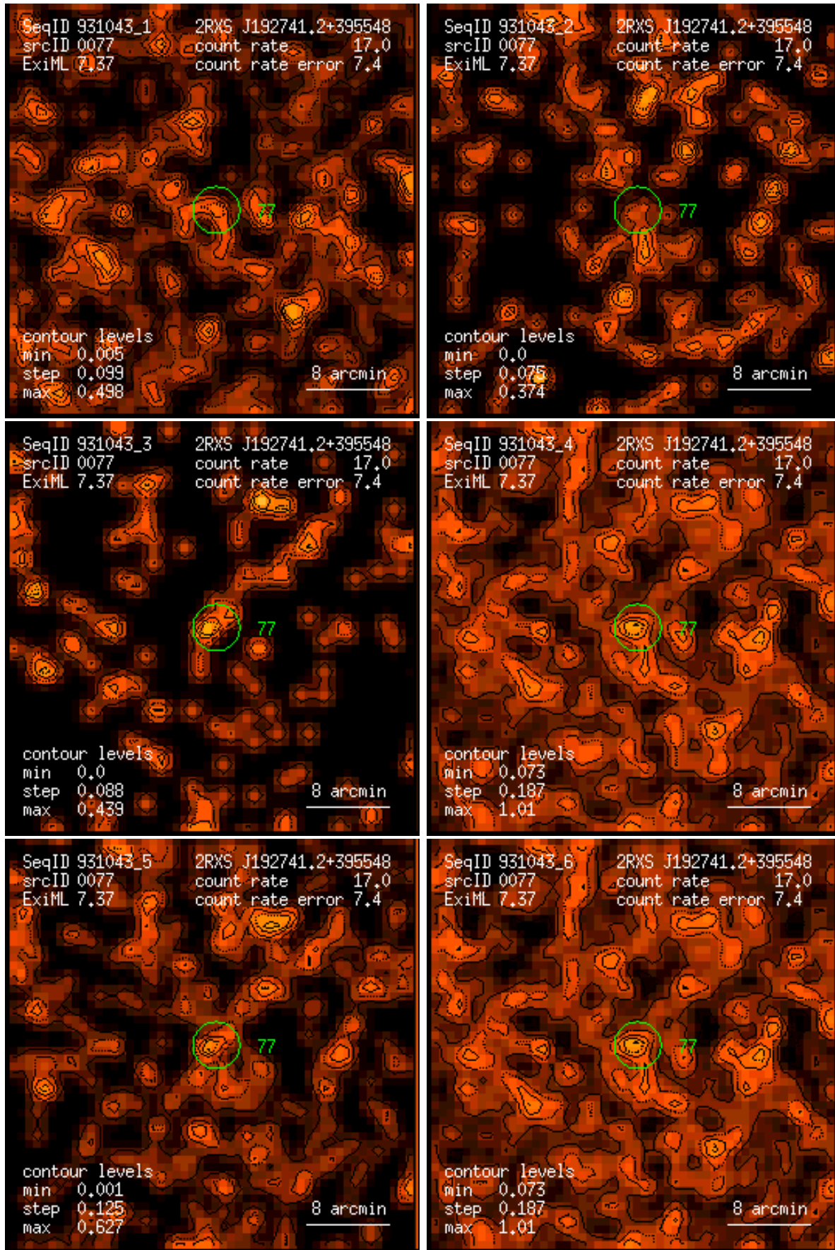
Figure 77: RASS 931043: detection 0077: band rate images, Gaussian filter: (1) PSPC channels 11 – 41, (2) 52 – 90, (3) 91 – 201, (4) 11 – 235, (5) 52 – 201, (6) 11 – 201. Broad band rates in counts/ks. Band rate contour levels in counts/ks/arcmin 2 .
