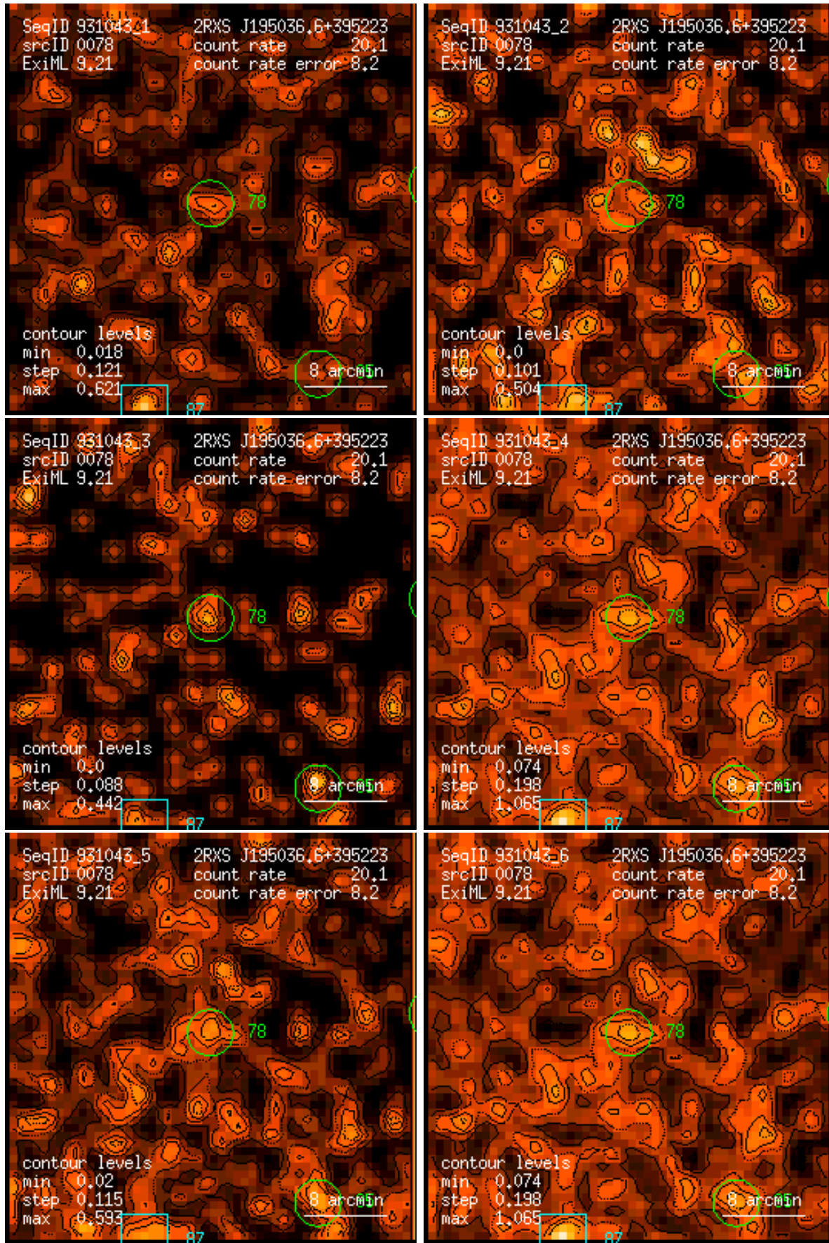
Figure 78: RASS 931043: detection 0078: band rate images, Gaussian filter: (1) PSPC channels 11 – 41, (2) 52 – 90, (3) 91 – 201, (4) 11 – 235, (5) 52 – 201, (6) 11 – 201. Broad band rates in counts/ks. Band rate contour levels in counts/ks/arcmin 2 .
