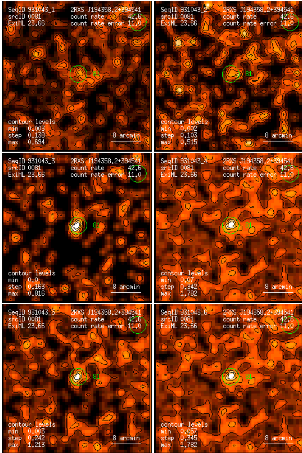
Figure 81: RASS 931043: detection 0081: band rate images, Gaussian filter: (1) PSPC channels 11 – 41, (2) 52 – 90, (3) 91 – 201, (4) 11 – 235, (5) 52 – 201, (6) 11 – 201. Broad band rates in counts/ks. Band rate contour levels in counts/ks/arcmin 2 .
