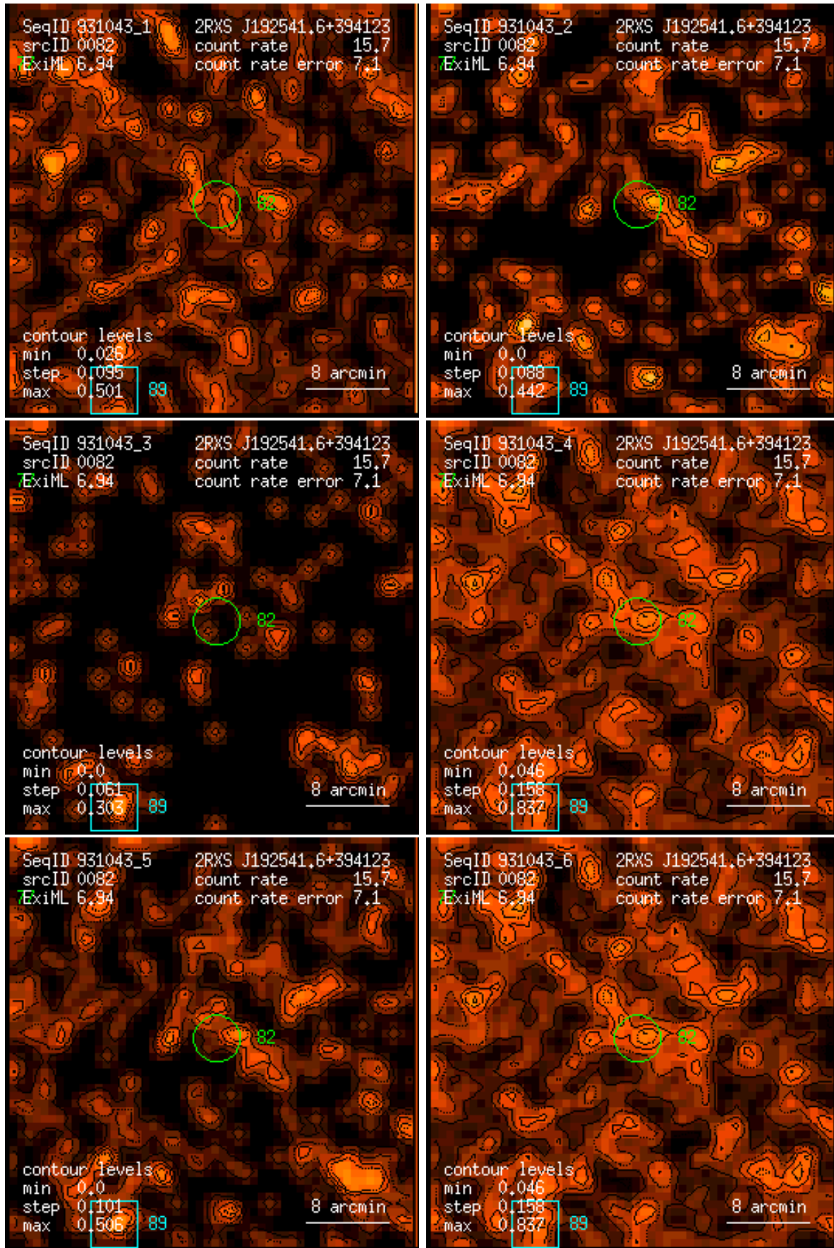
Figure 82: RASS 931043: detection 0082: band rate images, Gaussian filter: (1) PSPC channels 11 – 41, (2) 52 – 90, (3) 91 – 201, (4) 11 – 235, (5) 52 – 201, (6) 11 – 201. Broad band rates in counts/ks. Band rate contour levels in counts/ks/arcmin 2 .
