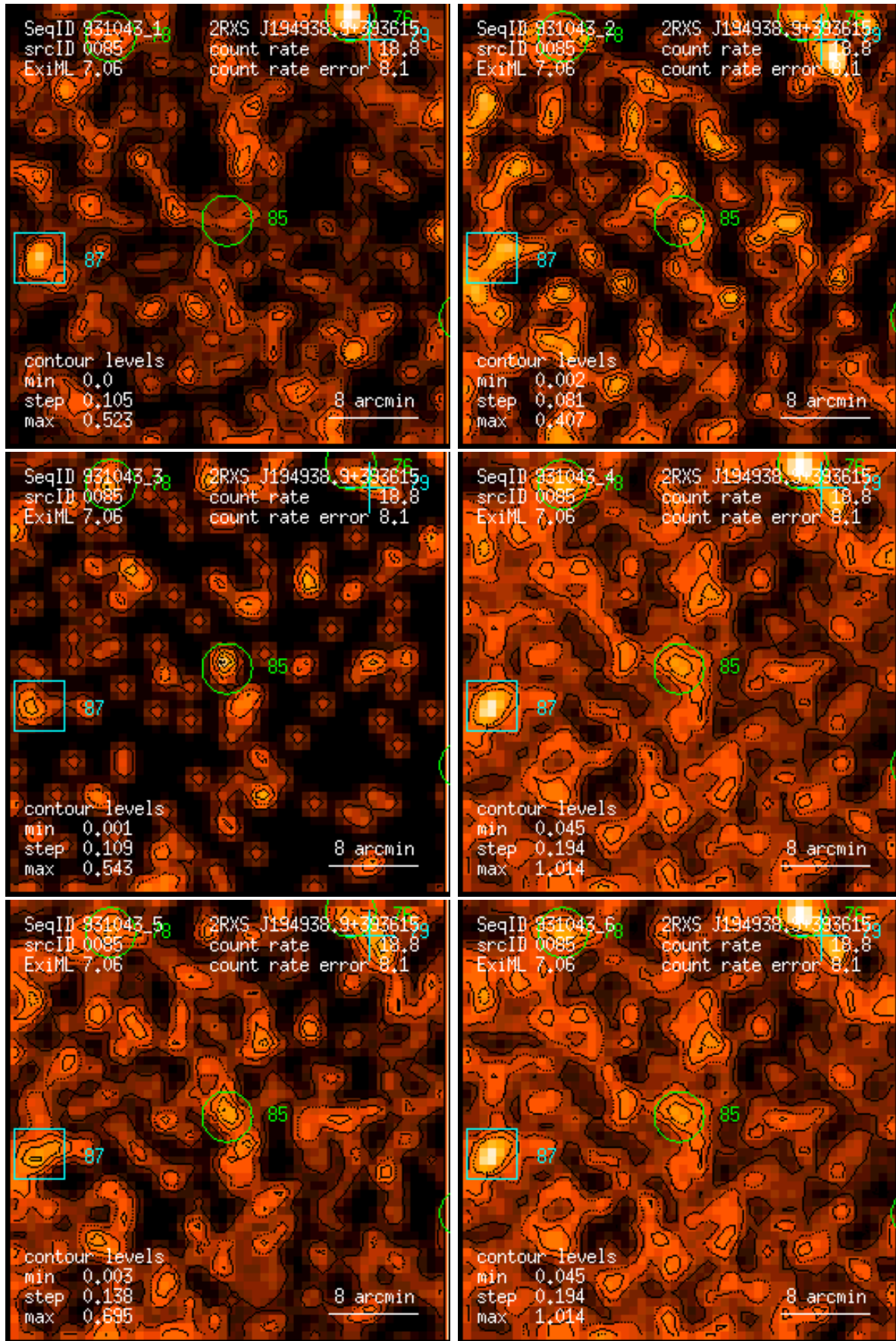
Figure 85: RASS 931043: detection 0085: band rate images, Gaussian filter: (1) PSPC channels 11 – 41, (2) 52 – 90, (3) 91 – 201, (4) 11 – 235, (5) 52 – 201, (6) 11 – 201. Broad band rates in counts/ks. Band rate contour levels in counts/ks/arcmin 2 .
