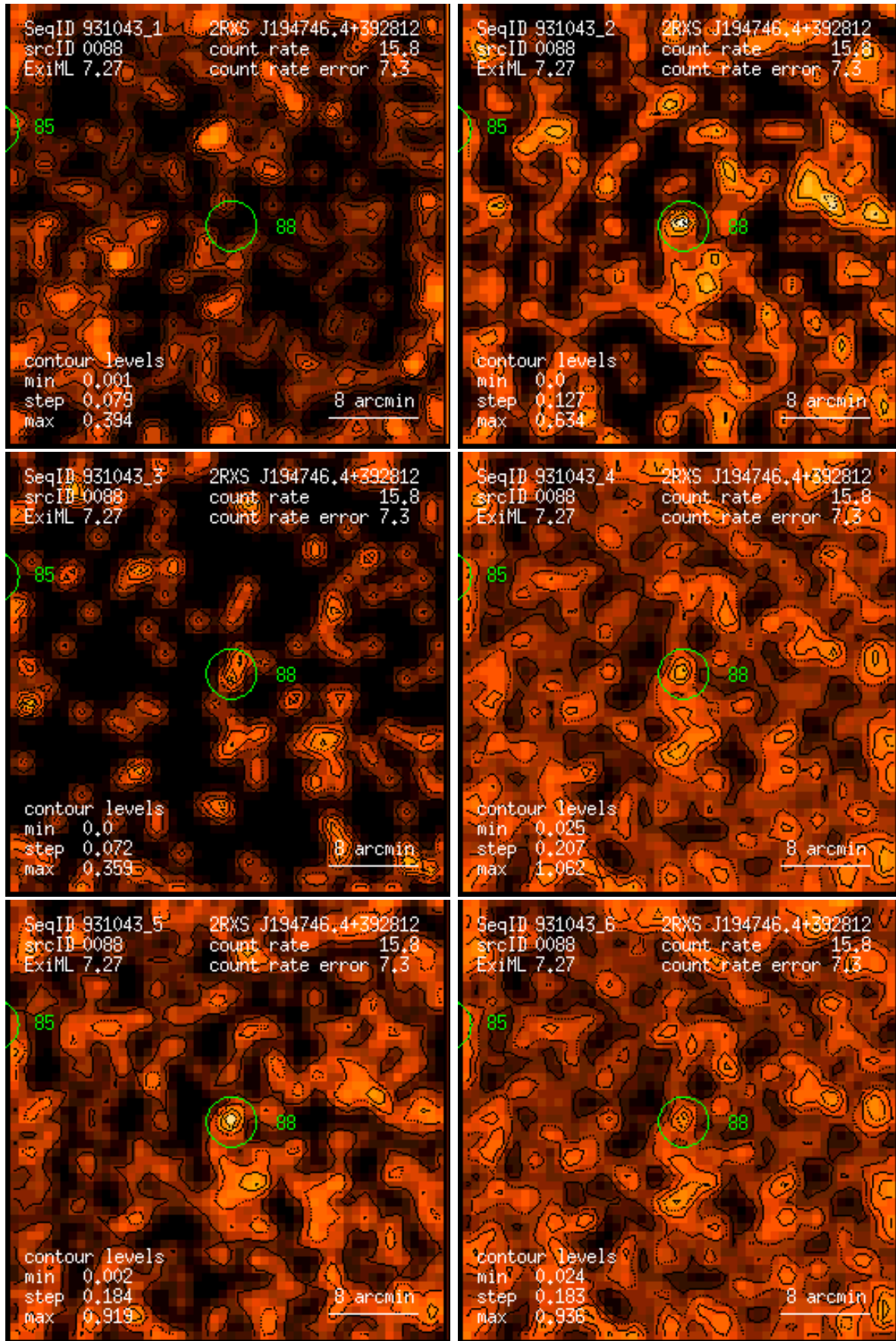
Figure 88: RASS 931043: detection 0088: band rate images, Gaussian filter: (1) PSPC channels 11 – 41, (2) 52 – 90, (3) 91 – 201, (4) 11 – 235, (5) 52 – 201, (6) 11 – 201. Broad band rates in counts/ks. Band rate contour levels in counts/ks/arcmin 2 .
