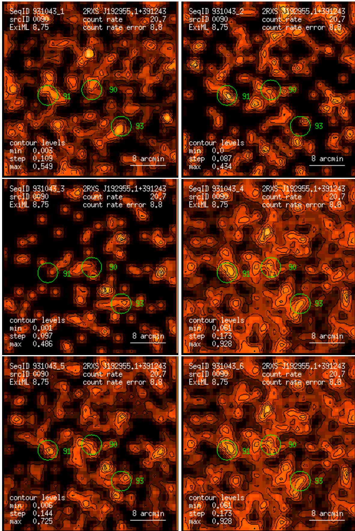
Figure 90: RASS 931043: detection 0090: band rate images, Gaussian filter: (1) PSPC channels 11 – 41, (2) 52 – 90, (3) 91 – 201, (4) 11 – 235, (5) 52 – 201, (6) 11 – 201. Broad band rates in counts/ks. Band rate contour levels in counts/ks/arcmin 2 .
