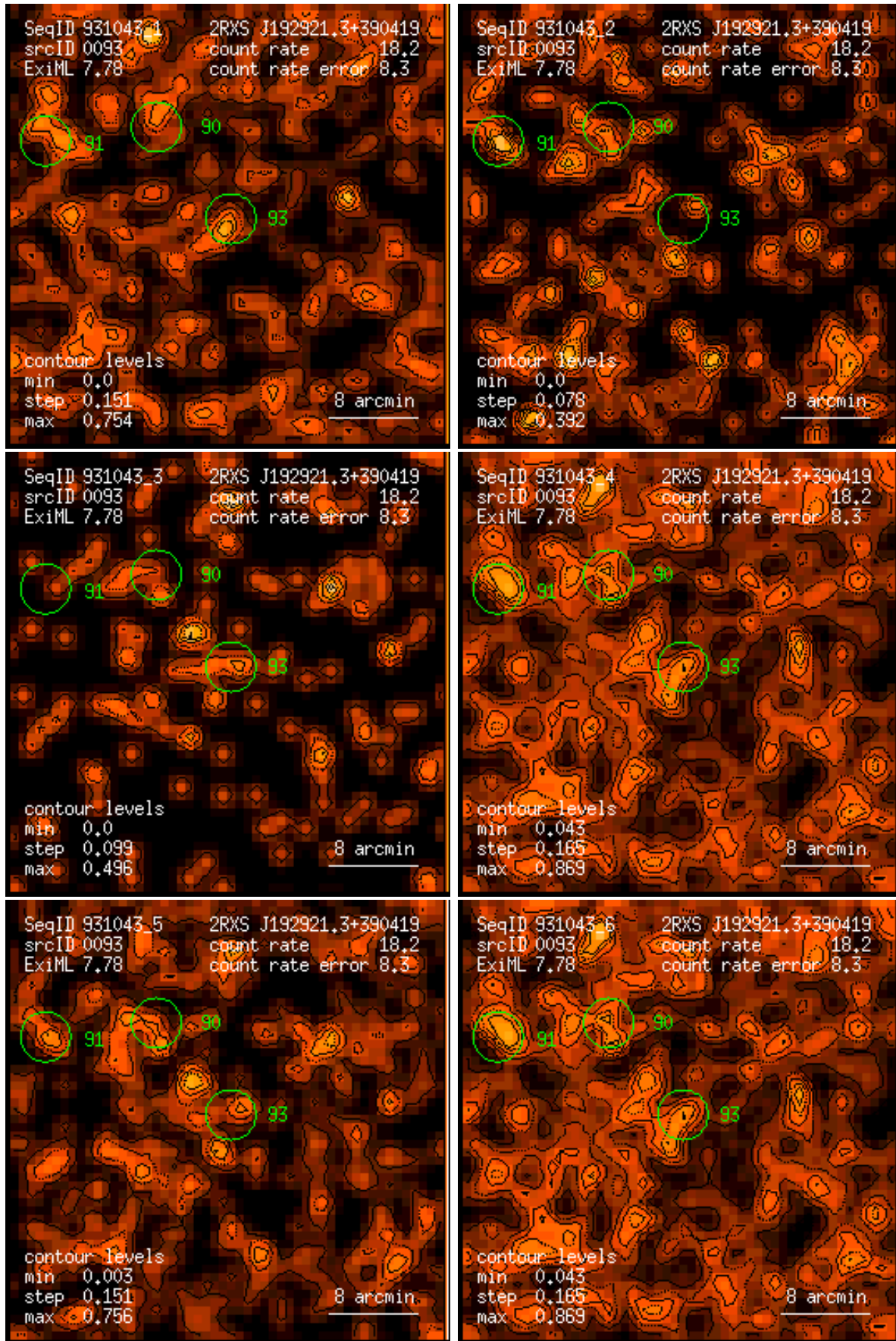
Figure 93: RASS 931043: detection 0093: band rate images, Gaussian filter: (1) PSPC channels 11 – 41, (2) 52 – 90, (3) 91 – 201, (4) 11 – 235, (5) 52 – 201, (6) 11 – 201. Broad band rates in counts/ks. Band rate contour levels in counts/ks/arcmin 2 .
