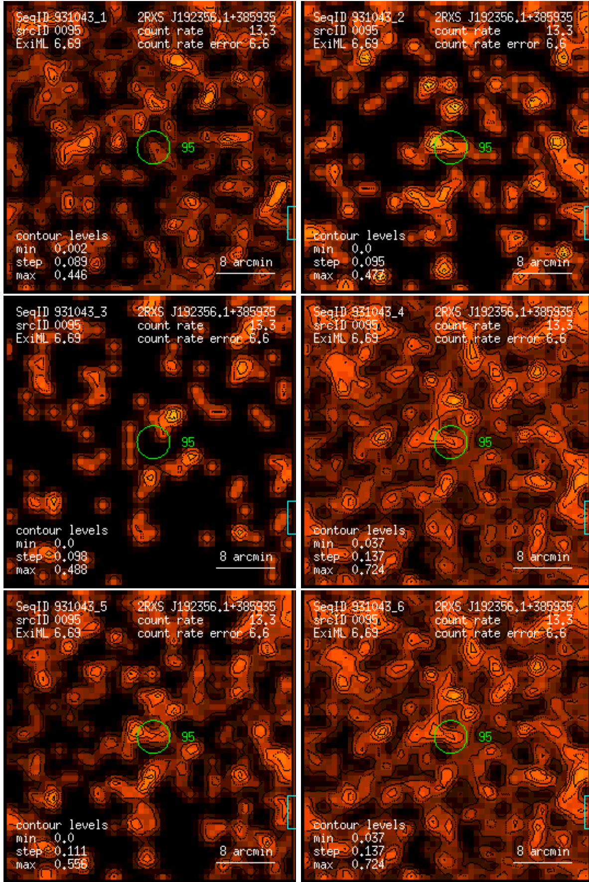
Figure 95: RASS 931043: detection 0095: band rate images, Gaussian filter: (1) PSPC channels 11 – 41, (2) 52 – 90, (3) 91 – 201, (4) 11 – 235, (5) 52 – 201, (6) 11 – 201. Broad band rates in counts/ks. Band rate contour levels in counts/ks/arcmin 2 .
