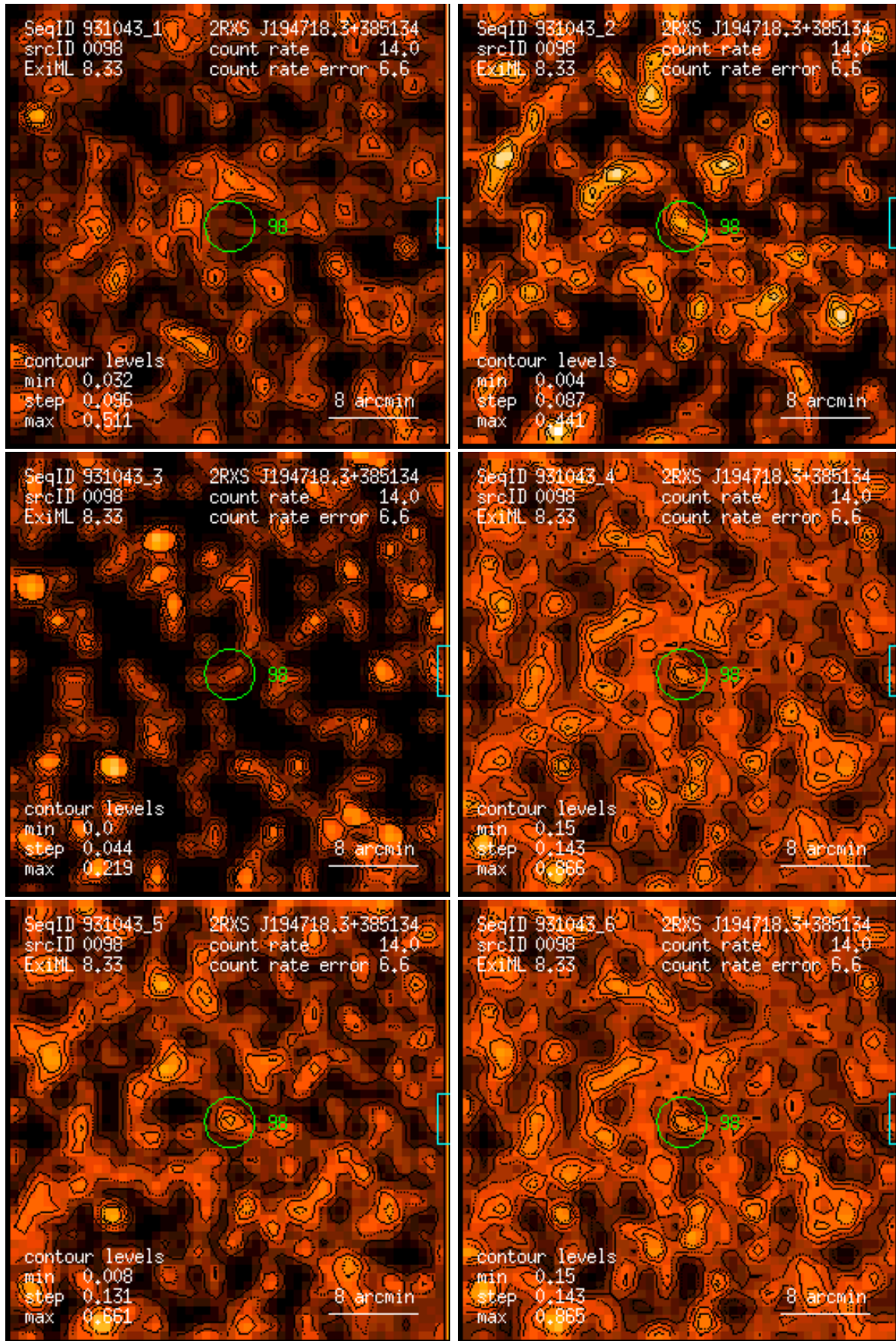
Figure 98: RASS 931043: detection 0098: band rate images, Gaussian filter: (1) PSPC channels 11 – 41, (2) 52 – 90, (3) 91 – 201, (4) 11 – 235, (5) 52 – 201, (6) 11 – 201. Broad band rates in counts/ks. Band rate contour levels in counts/ks/arcmin 2 .
