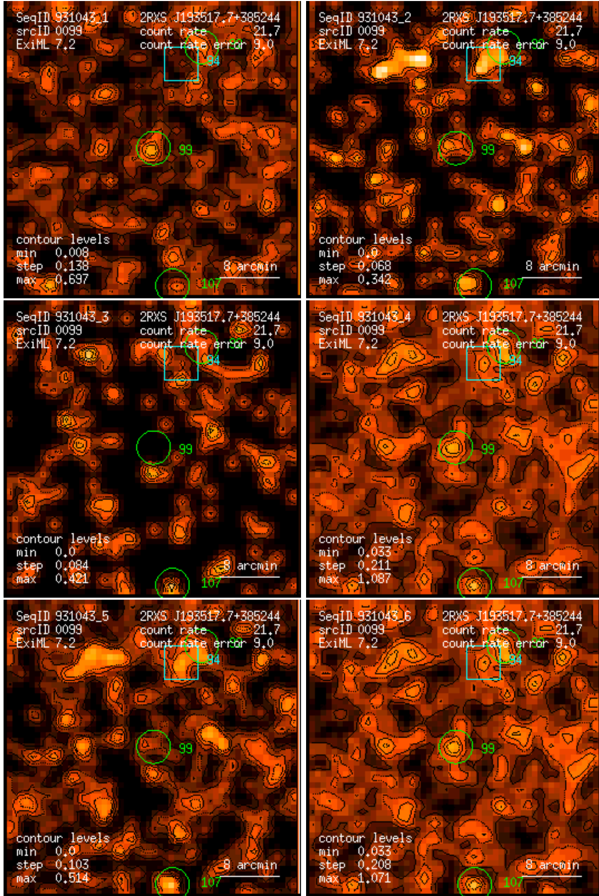
Figure 99: RASS 931043: detection 0099: band rate images, Gaussian filter: (1) PSPC channels 11 – 41, (2) 52 – 90, (3) 91 – 201, (4) 11 – 235, (5) 52 – 201, (6) 11 – 201. Broad band rates in counts/ks. Band rate contour levels in counts/ks/arcmin 2 .
