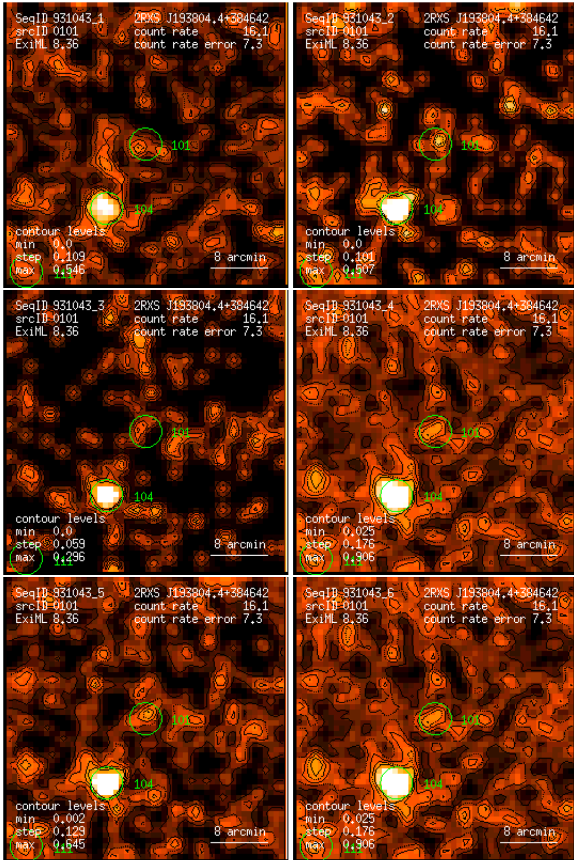
Figure 101: RASS 931043: detection 0101: band rate images, Gaussian filter: (1) PSPC channels 11 – 41, (2) 52 – 90, (3) 91 – 201, (4) 11 – 235, (5) 52 – 201, (6) 11 – 201. Broad band rates in counts/ks. Band rate contour levels in counts/ks/arcmin 2 .
