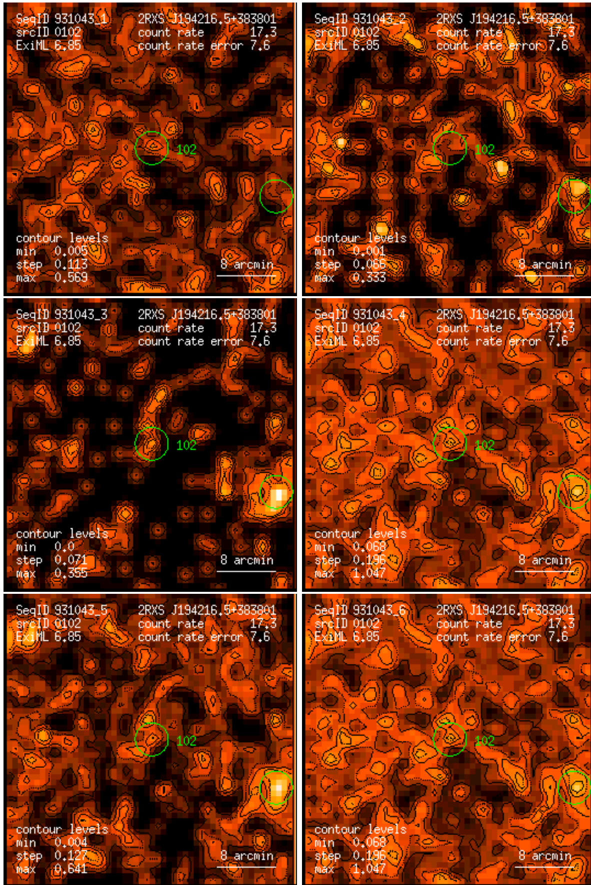
Figure 102: RASS 931043: detection 0102: band rate images, Gaussian filter: (1) PSPC channels 11 – 41, (2) 52 – 90, (3) 91 – 201, (4) 11 – 235, (5) 52 – 201, (6) 11 – 201. Broad band rates in counts/ks. Band rate contour levels in counts/ks/arcmin 2 .
