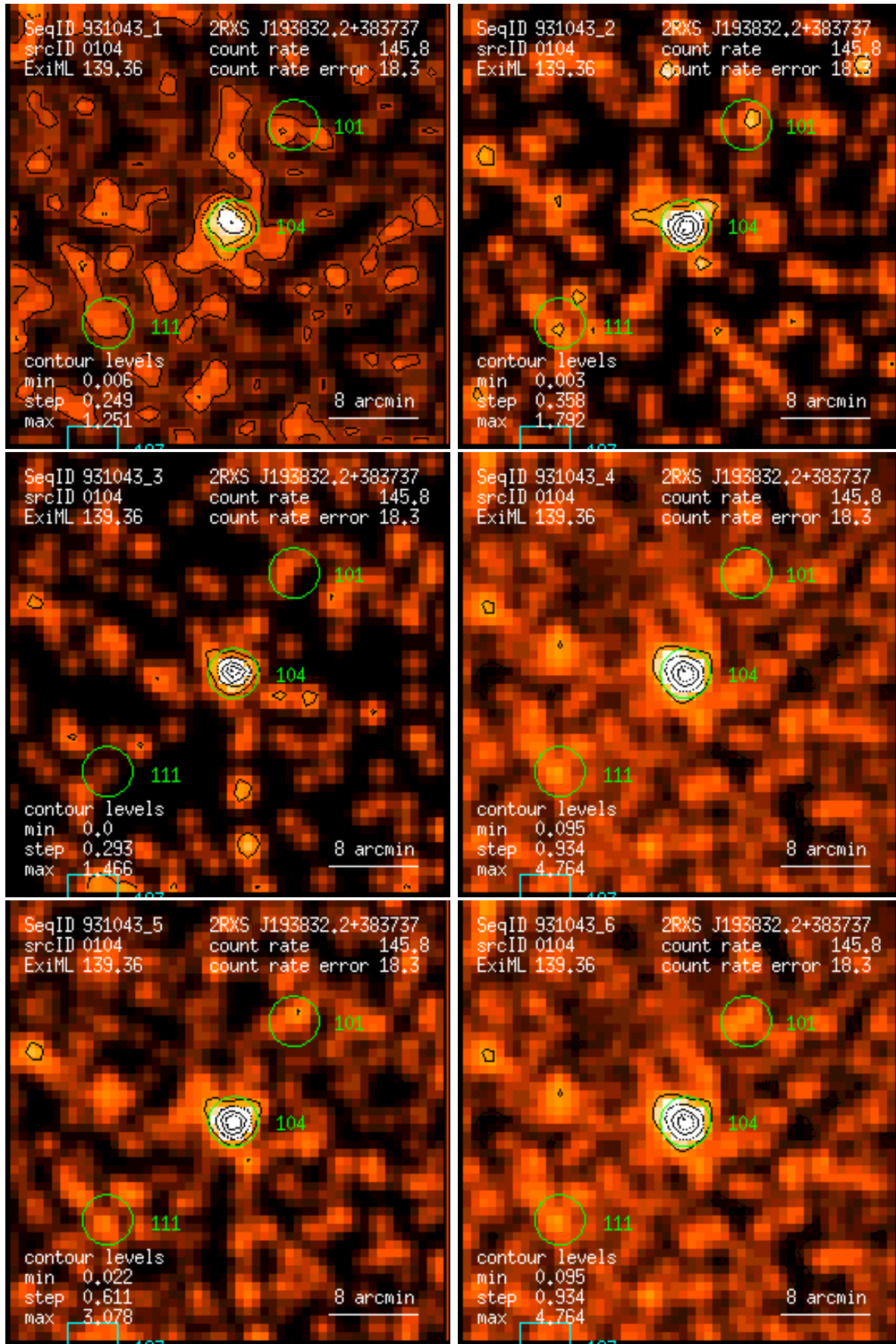
Figure 104: RASS 931043: detection 0104: band rate images, Gaussian filter: (1) PSPC channels 11 – 41, (2) 52 – 90, (3) 91 – 201, (4) 11 – 235, (5) 52 – 201, (6) 11 – 201. Broad band rates in counts/ks. Band rate contour levels in counts/ks/arcmin 2 .
