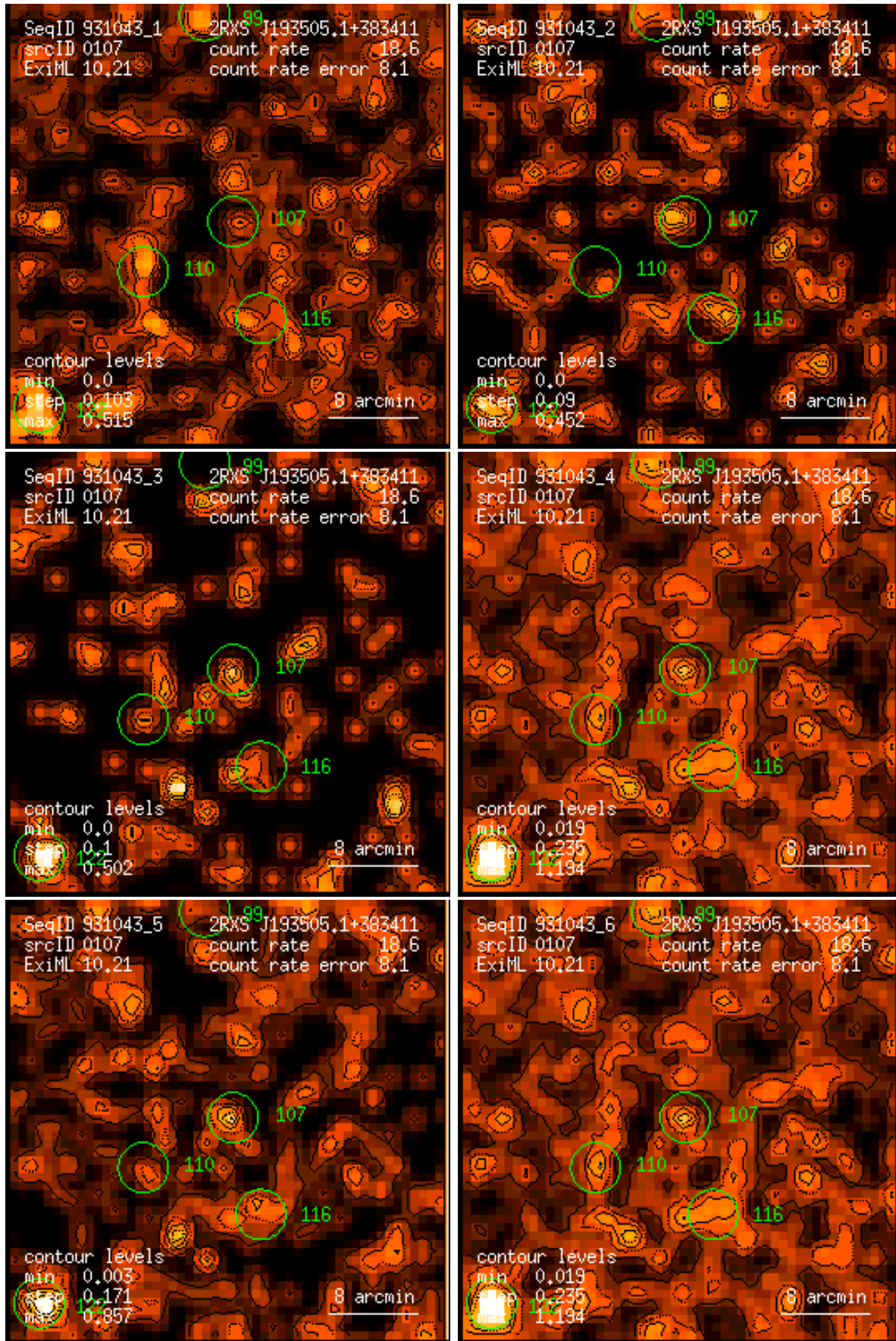
Figure 107: RASS 931043: detection 0107: band rate images, Gaussian filter: (1) PSPC channels 11 – 41, (2) 52 – 90, (3) 91 – 201, (4) 11 – 235, (5) 52 – 201, (6) 11 – 201. Broad band rates in counts/ks. Band rate contour levels in counts/ks/arcmin 2 .
