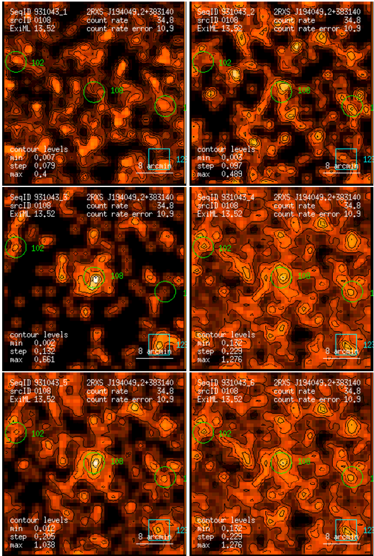
Figure 108: RASS 931043: detection 0108: band rate images, Gaussian filter: (1) PSPC channels 11 – 41, (2) 52 – 90, (3) 91 – 201, (4) 11 – 235, (5) 52 – 201, (6) 11 – 201. Broad band rates in counts/ks. Band rate contour levels in counts/ks/arcmin 2 .
