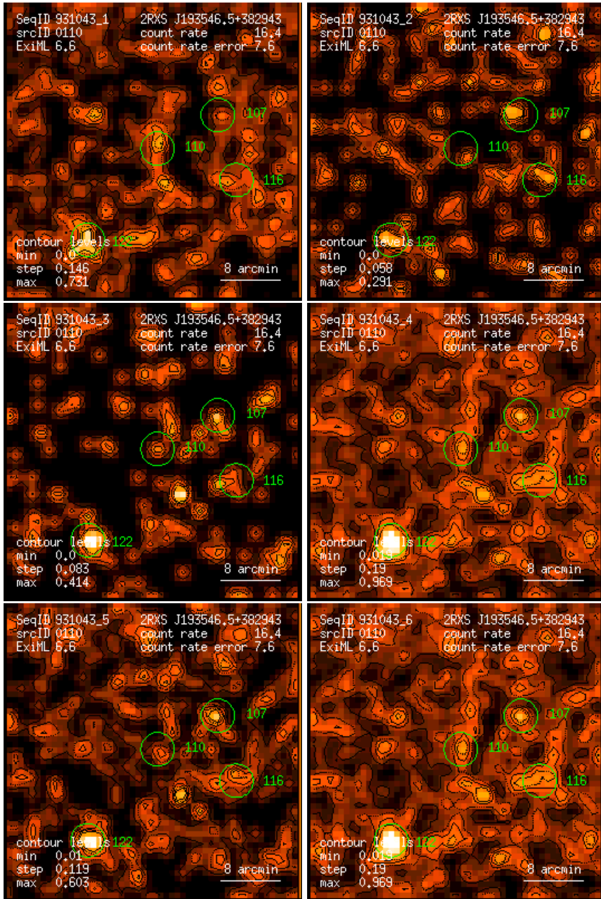
Figure 110: RASS 931043: detection 0110: band rate images, Gaussian filter: (1) PSPC channels 11 – 41, (2) 52 – 90, (3) 91 – 201, (4) 11 – 235, (5) 52 – 201, (6) 11 – 201. Broad band rates in counts/ks. Band rate contour levels in counts/ks/arcmin 2 .
