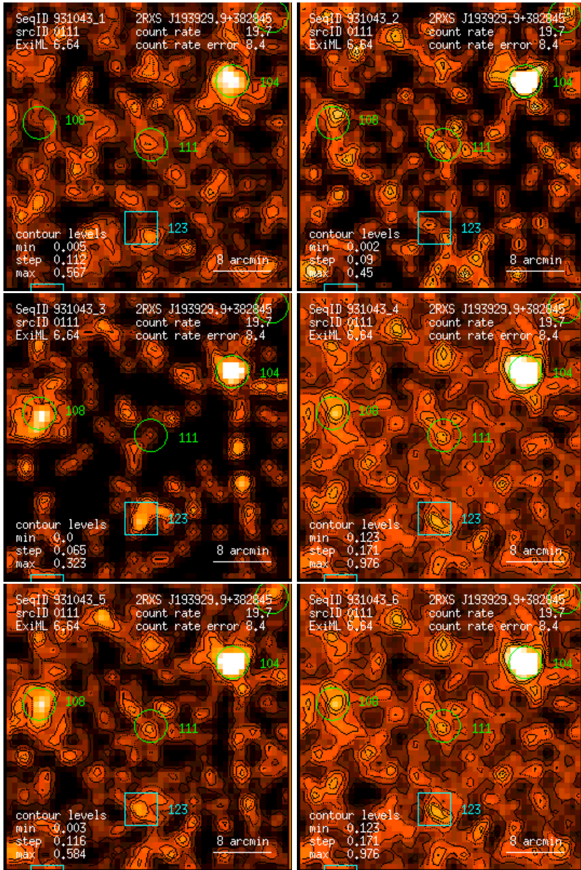
Figure 111: RASS 931043: detection 0111: band rate images, Gaussian filter: (1) PSPC channels 11 – 41, (2) 52 – 90, (3) 91 – 201, (4) 11 – 235, (5) 52 – 201, (6) 11 – 201. Broad band rates in counts/ks. Band rate contour levels in counts/ks/arcmin 2 .
