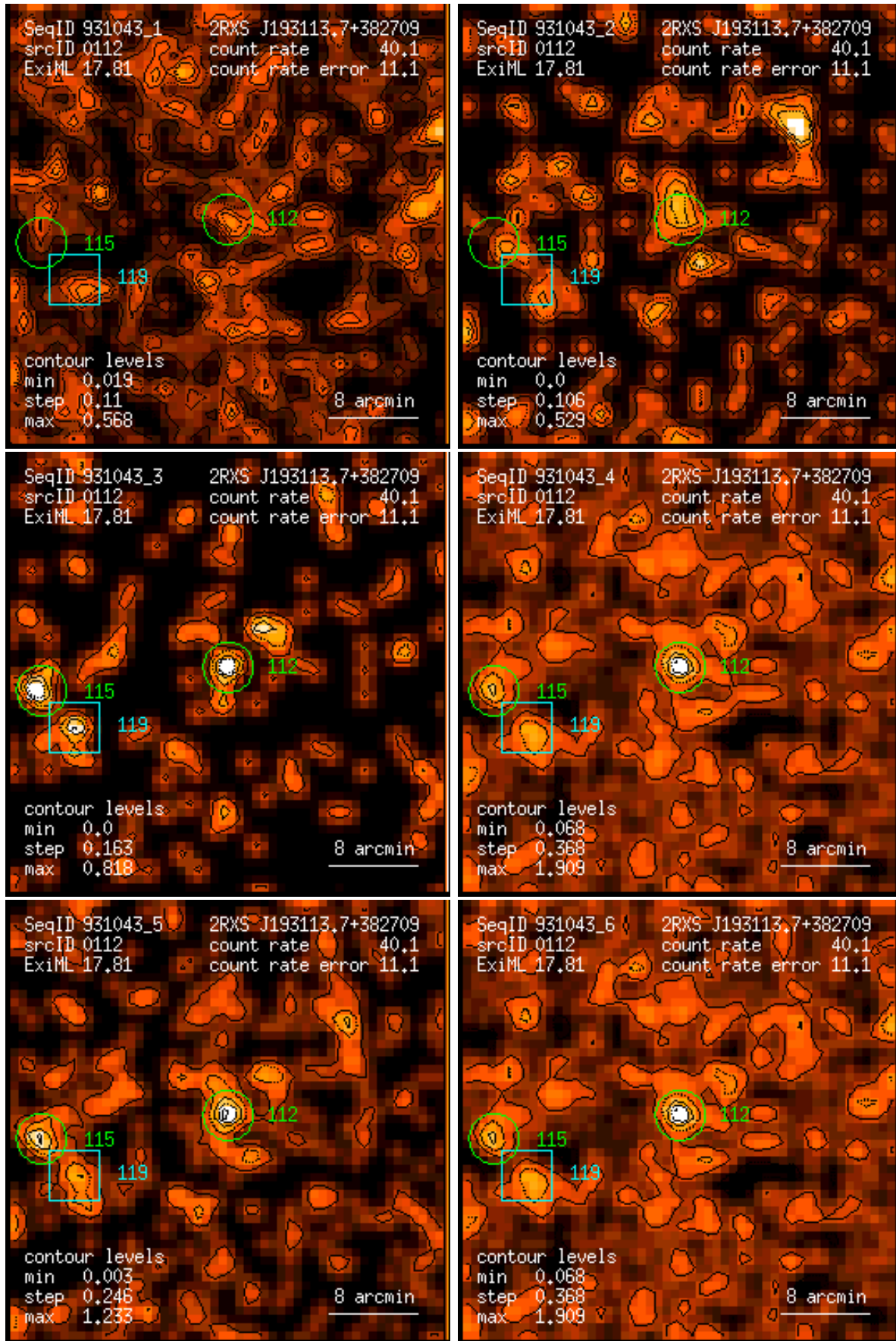
Figure 112: RASS 931043: detection 0112: band rate images, Gaussian filter: (1) PSPC channels 11 – 41, (2) 52 – 90, (3) 91 – 201, (4) 11 – 235, (5) 52 – 201, (6) 11 – 201. Broad band rates in counts/ks. Band rate contour levels in counts/ks/arcmin 2 .
