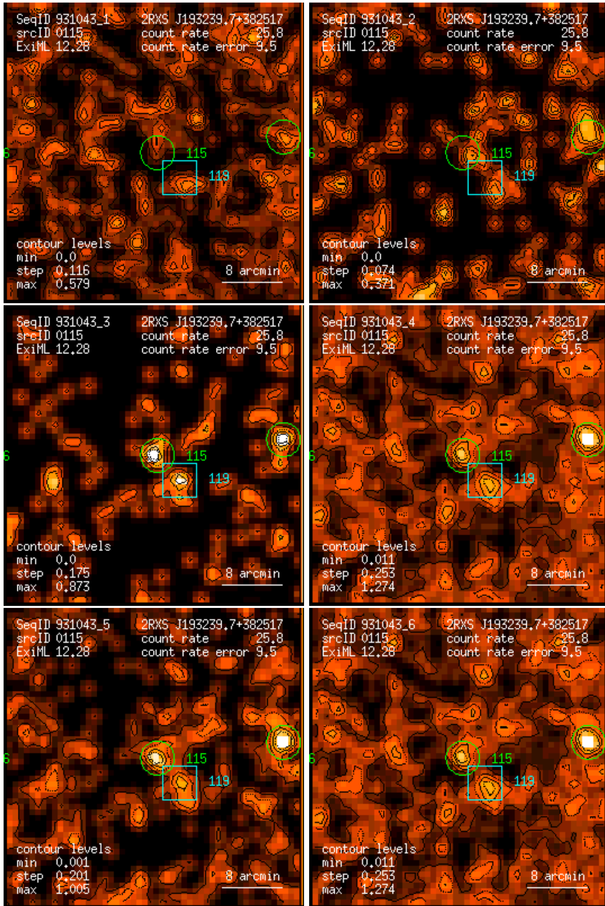
Figure 115: RASS 931043: detection 0115: band rate images, Gaussian filter: (1) PSPC channels 11 – 41, (2) 52 – 90, (3) 91 – 201, (4) 11 – 235, (5) 52 – 201, (6) 11 – 201. Broad band rates in counts/ks. Band rate contour levels in counts/ks/arcmin 2 .
