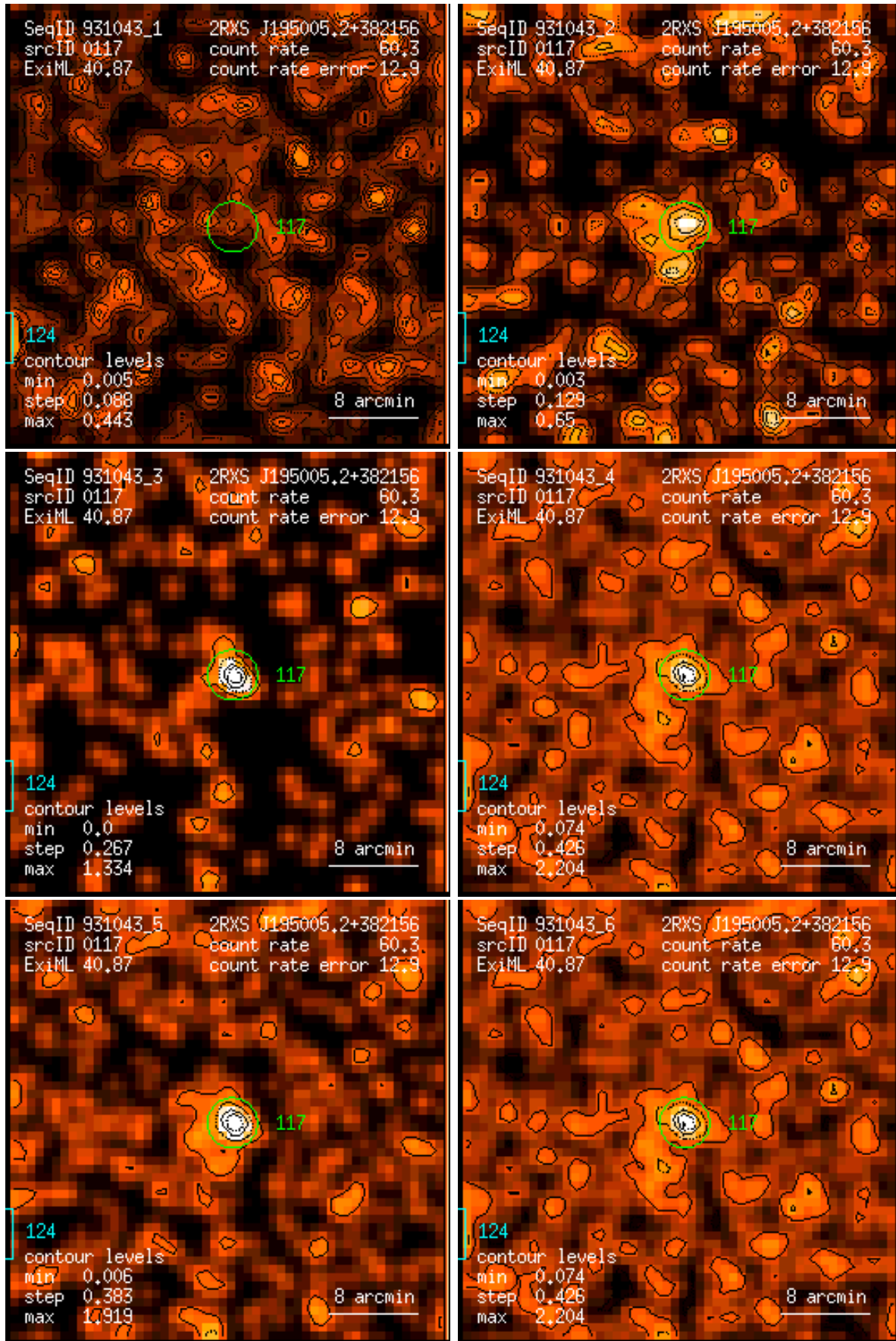
Figure 117: RASS 931043: detection 0117: band rate images, Gaussian filter: (1) PSPC channels 11 – 41, (2) 52 – 90, (3) 91 – 201, (4) 11 – 235, (5) 52 – 201, (6) 11 – 201. Broad band rates in counts/ks. Band rate contour levels in counts/ks/arcmin 2 .
