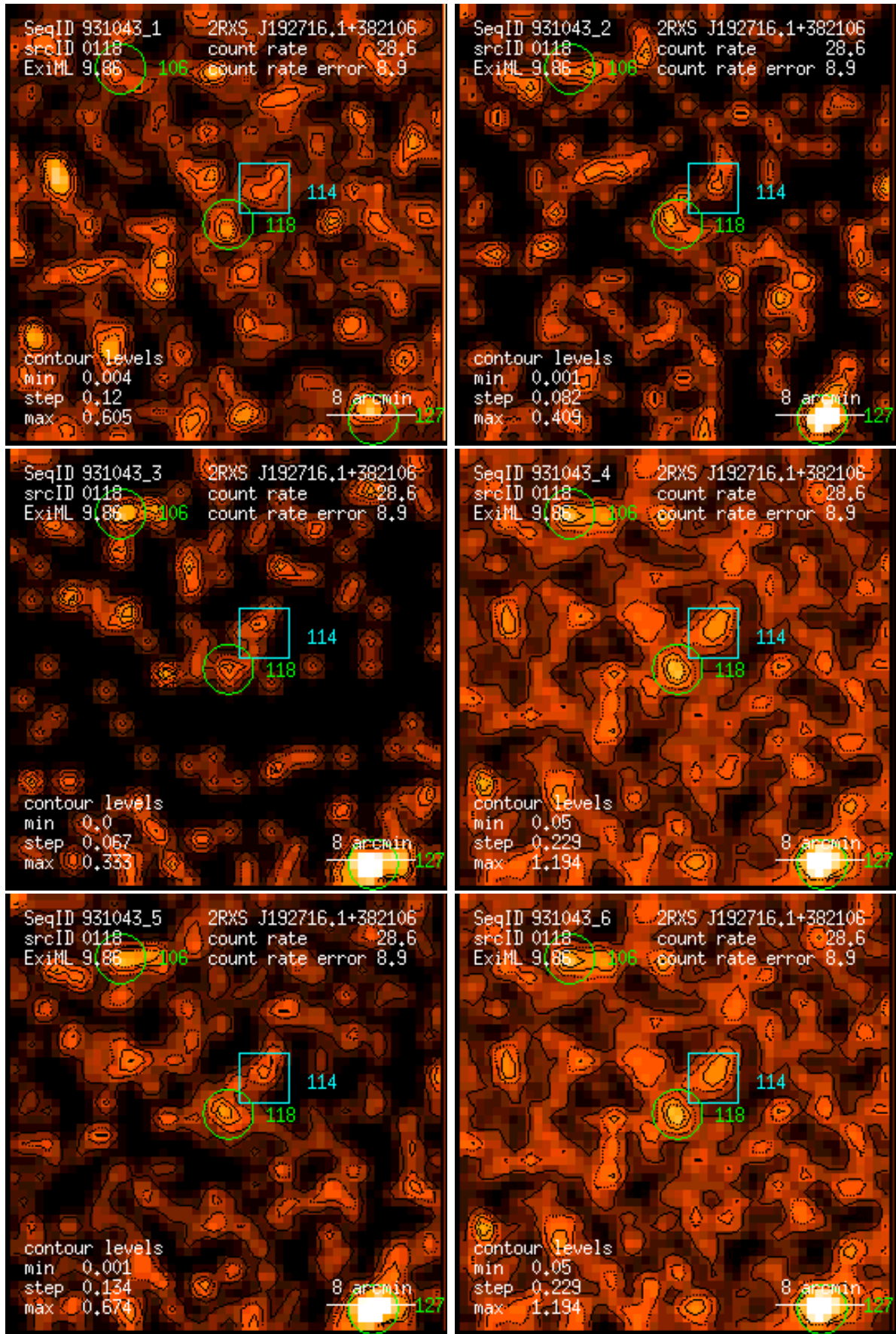
Figure 118: RASS 931043: detection 0118: band rate images, Gaussian filter: (1) PSPC channels 11 – 41, (2) 52 – 90, (3) 91 – 201, (4) 11 – 235, (5) 52 – 201, (6) 11 – 201. Broad band rates in counts/ks. Band rate contour levels in counts/ks/arcmin 2 .
