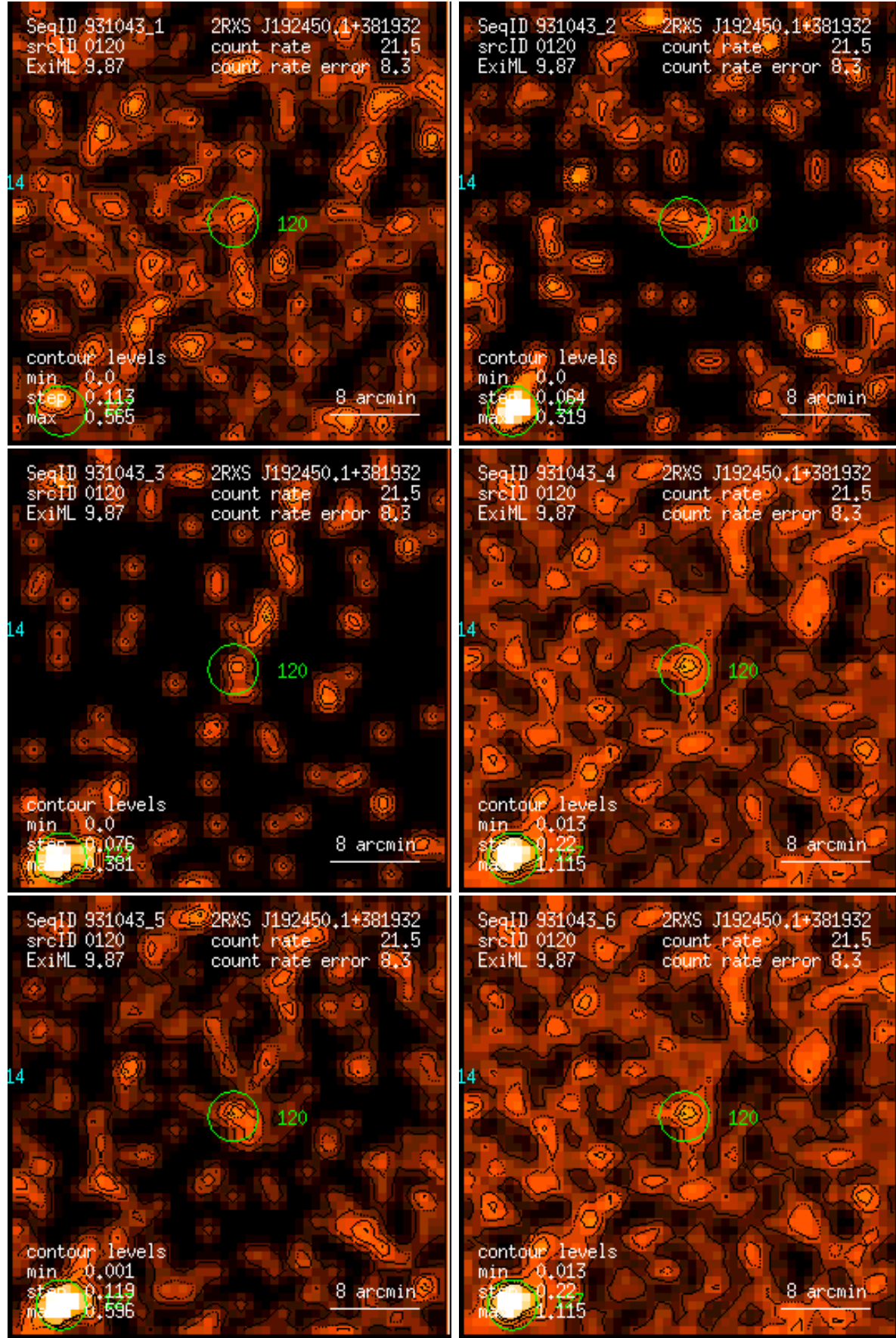
Figure 120: RASS 931043: detection 0120: band rate images, Gaussian filter: (1) PSPC channels 11 – 41, (2) 52 – 90, (3) 91 – 201, (4) 11 – 235, (5) 52 – 201, (6) 11 – 201. Broad band rates in counts/ks. Band rate contour levels in counts/ks/arcmin 2 .
