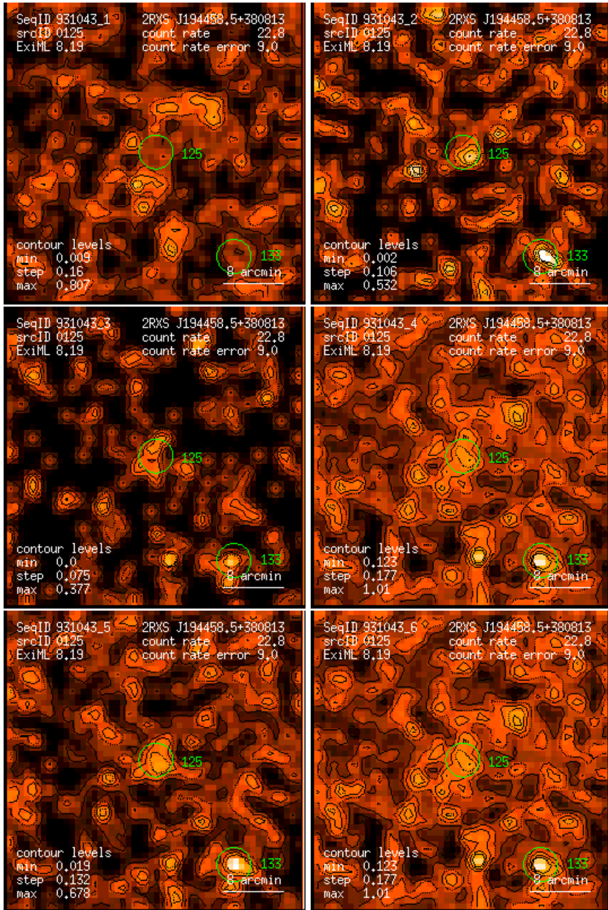
Figure 125: RASS 931043: detection 0125: band rate images, Gaussian filter: (1) PSPC channels 11 – 41, (2) 52 – 90, (3) 91 – 201, (4) 11 – 235, (5) 52 – 201, (6) 11 – 201. Broad band rates in counts/ks. Band rate contour levels in counts/ks/arcmin 2 .
