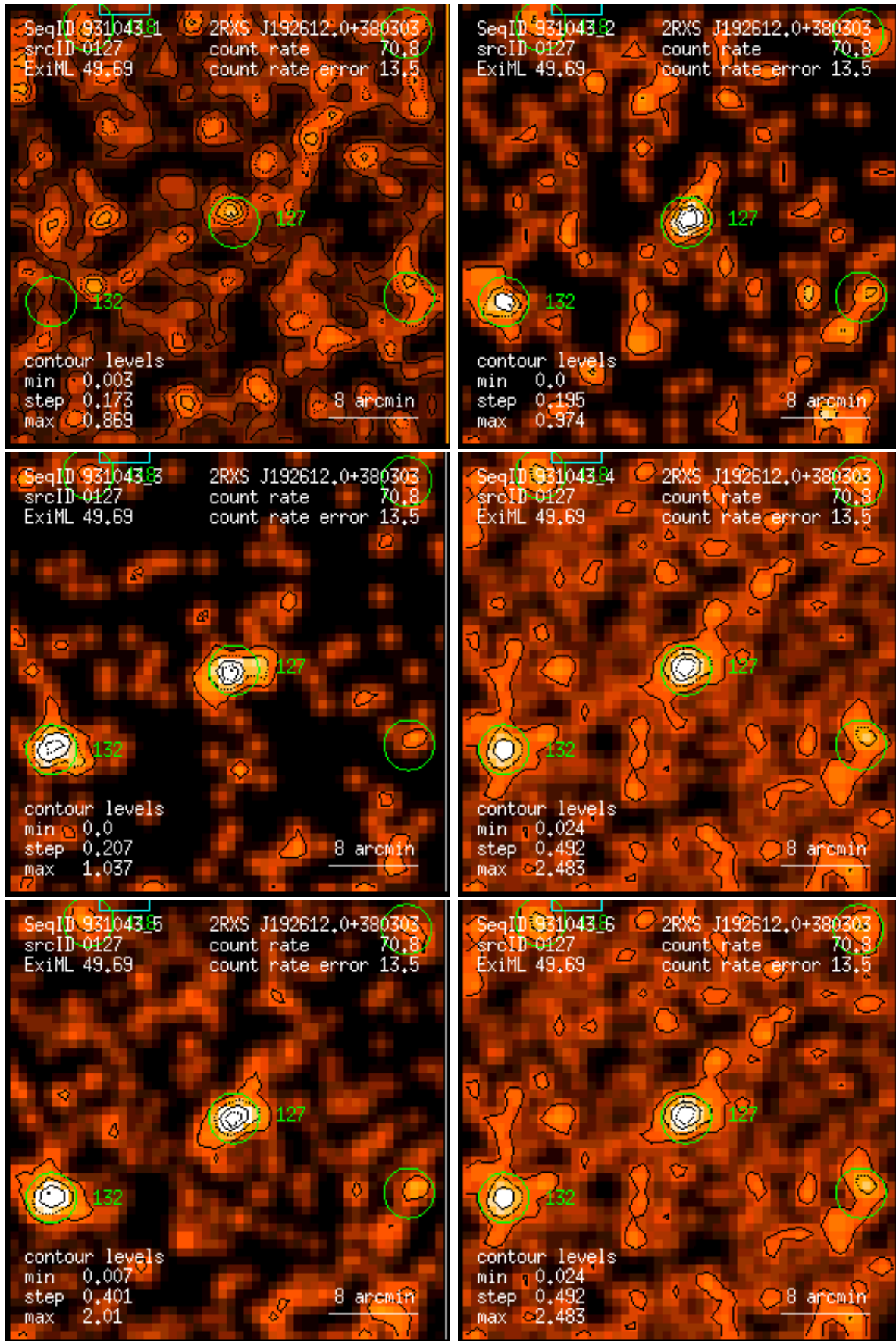
Figure 127: RASS 931043: detection 0127: band rate images, Gaussian filter: (1) PSPC channels 11 – 41, (2) 52 – 90, (3) 91 – 201, (4) 11 – 235, (5) 52 – 201, (6) 11 – 201. Broad band rates in counts/ks. Band rate contour levels in counts/ks/arcmin 2 .
