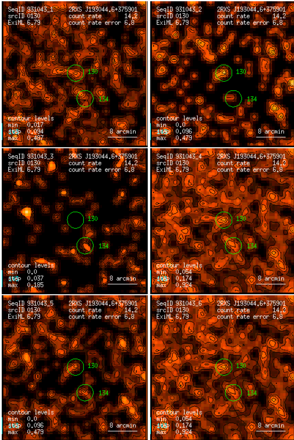
Figure 130: RASS 931043: detection 0130: band rate images, Gaussian filter: (1) PSPC channels 11 – 41, (2) 52 – 90, (3) 91 – 201, (4) 11 – 235, (5) 52 – 201, (6) 11 – 201. Broad band rates in counts/ks. Band rate contour levels in counts/ks/arcmin 2 .
