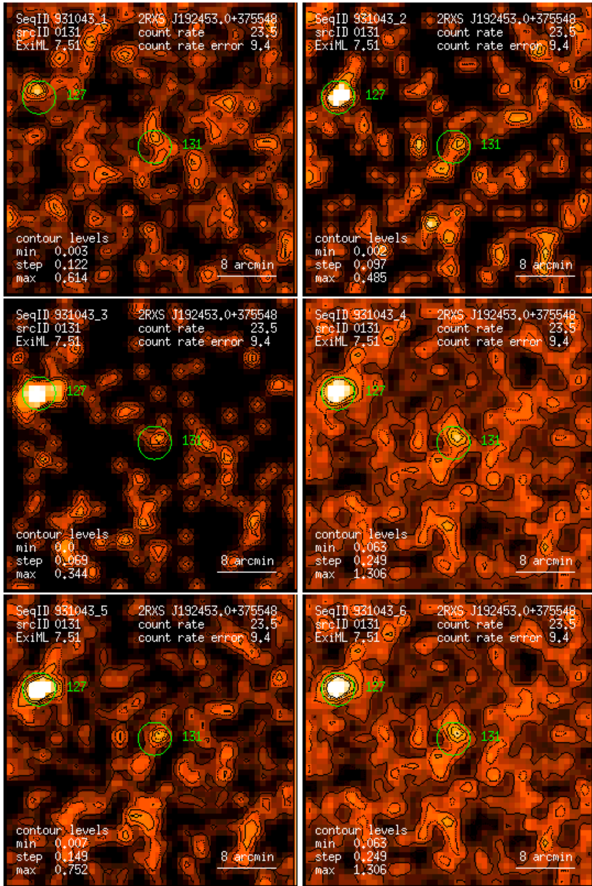
Figure 131: RASS 931043: detection 0131: band rate images, Gaussian filter: (1) PSPC channels 11 – 41, (2) 52 – 90, (3) 91 – 201, (4) 11 – 235, (5) 52 – 201, (6) 11 – 201. Broad band rates in counts/ks. Band rate contour levels in counts/ks/arcmin 2 .
