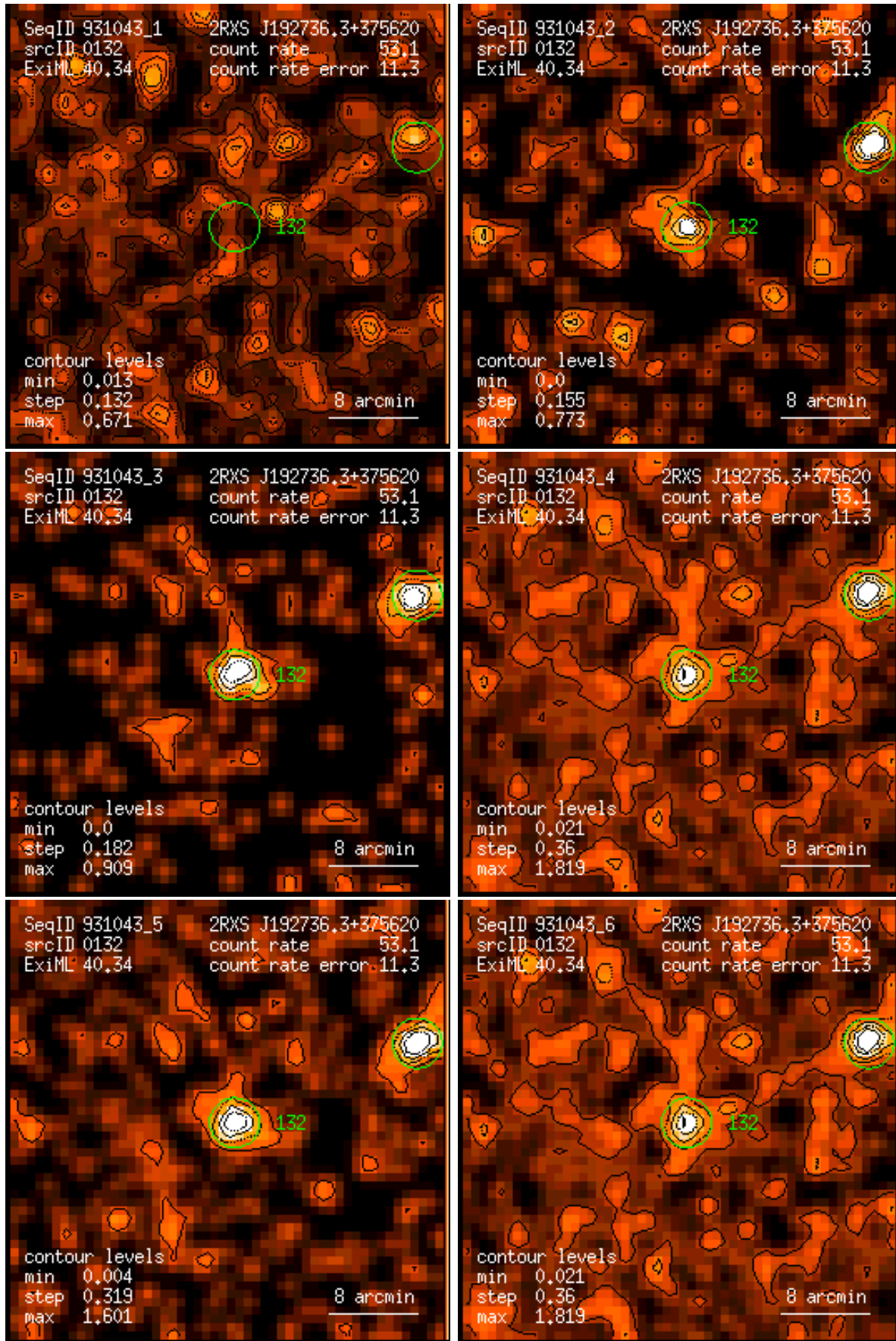
Figure 132: RASS 931043: detection 0132: band rate images, Gaussian filter: (1) PSPC channels 11 – 41, (2) 52 – 90, (3) 91 – 201, (4) 11 – 235, (5) 52 – 201, (6) 11 – 201. Broad band rates in counts/ks. Band rate contour levels in counts/ks/arcmin 2 .
