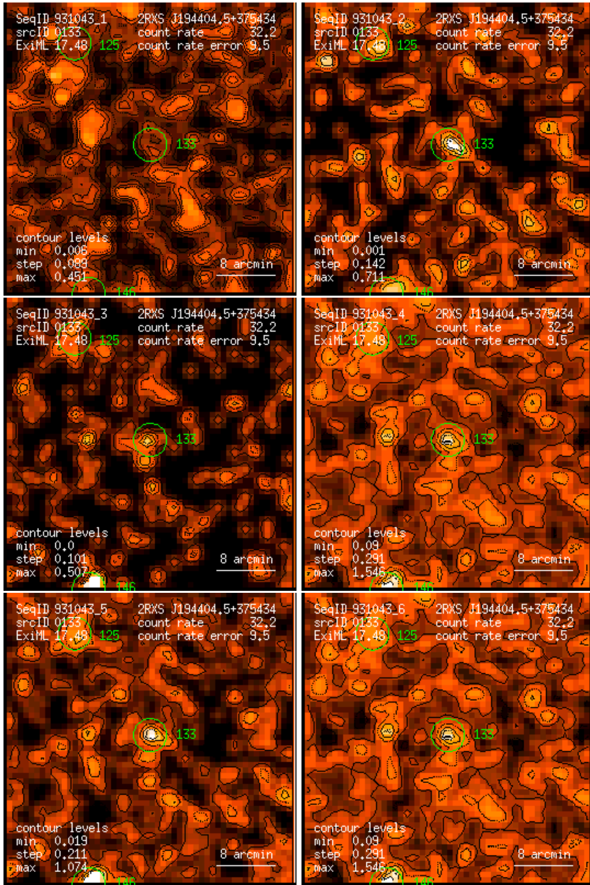
Figure 133: RASS 931043: detection 0133: band rate images, Gaussian filter: (1) PSPC channels 11 – 41, (2) 52 – 90, (3) 91 – 201, (4) 11 – 235, (5) 52 – 201, (6) 11 – 201. Broad band rates in counts/ks. Band rate contour levels in counts/ks/arcmin 2 .
