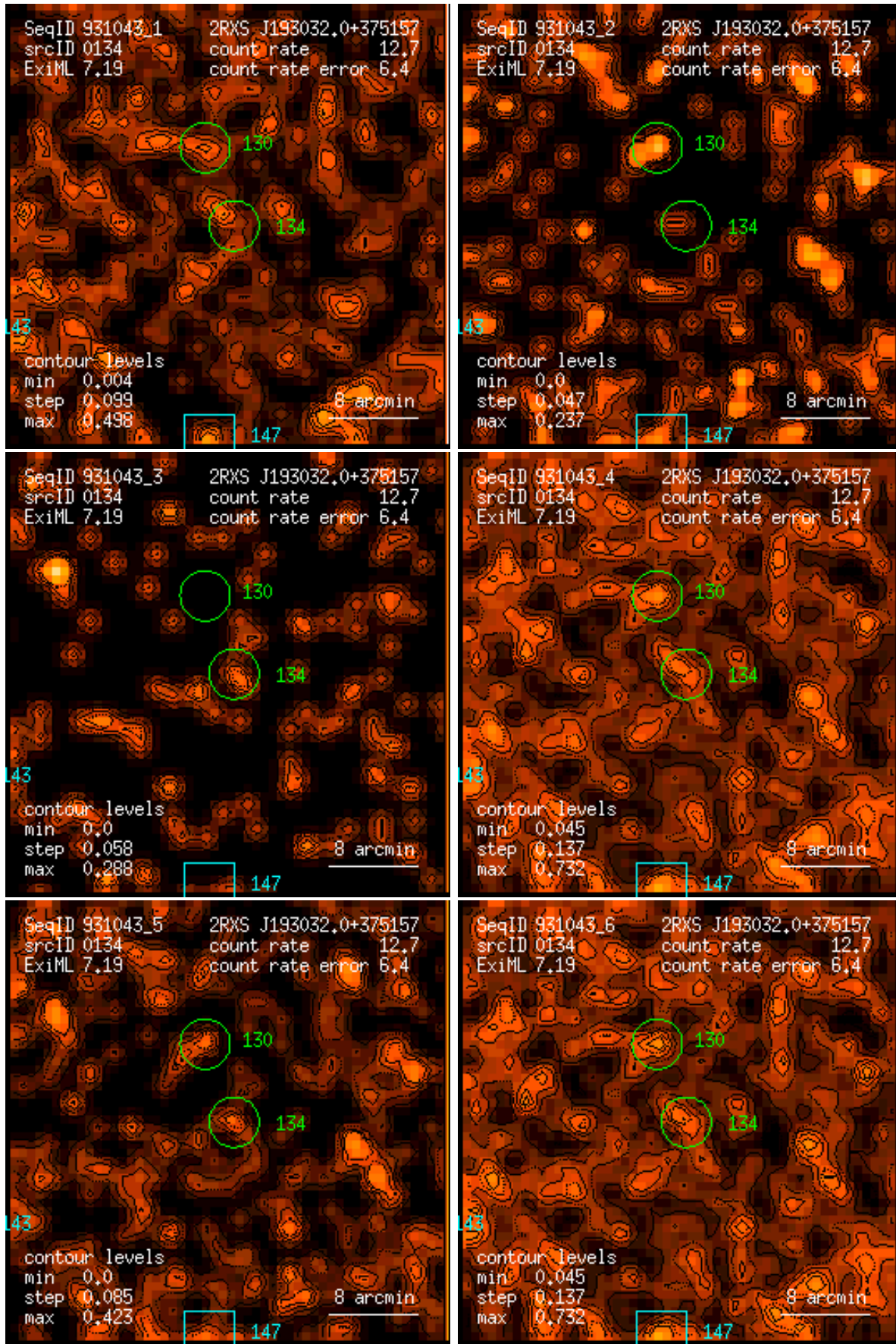
Figure 134: RASS 931043: detection 0134: band rate images, Gaussian filter: (1) PSPC channels 11 – 41, (2) 52 – 90, (3) 91 – 201, (4) 11 – 235, (5) 52 – 201, (6) 11 – 201. Broad band rates in counts/ks. Band rate contour levels in counts/ks/arcmin 2 .
