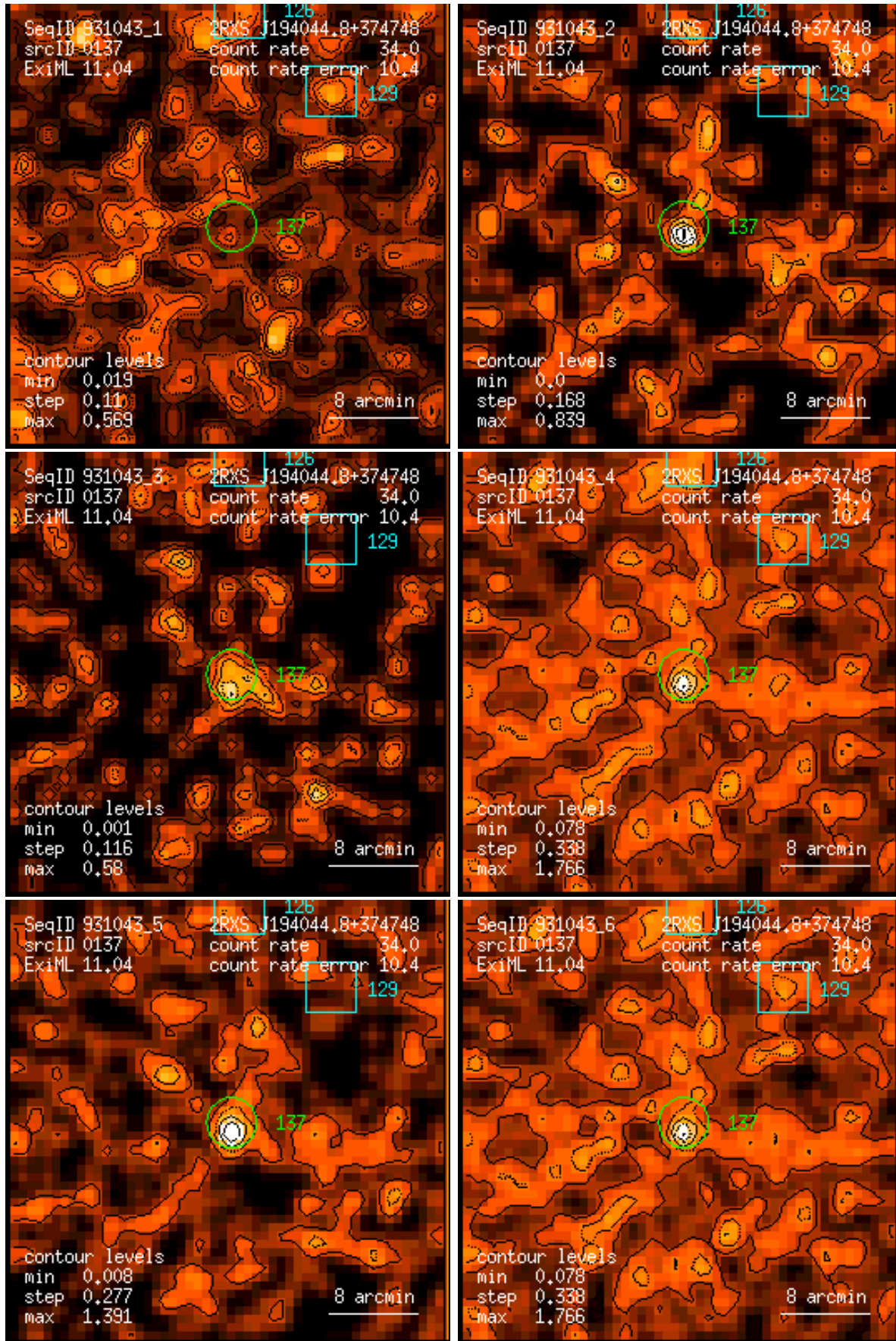
Figure 137: RASS 931043: detection 0137: band rate images, Gaussian filter: (1) PSPC channels 11 – 41, (2) 52 – 90, (3) 91 – 201, (4) 11 – 235, (5) 52 – 201, (6) 11 – 201. Broad band rates in counts/ks. Band rate contour levels in counts/ks/arcmin 2 .
