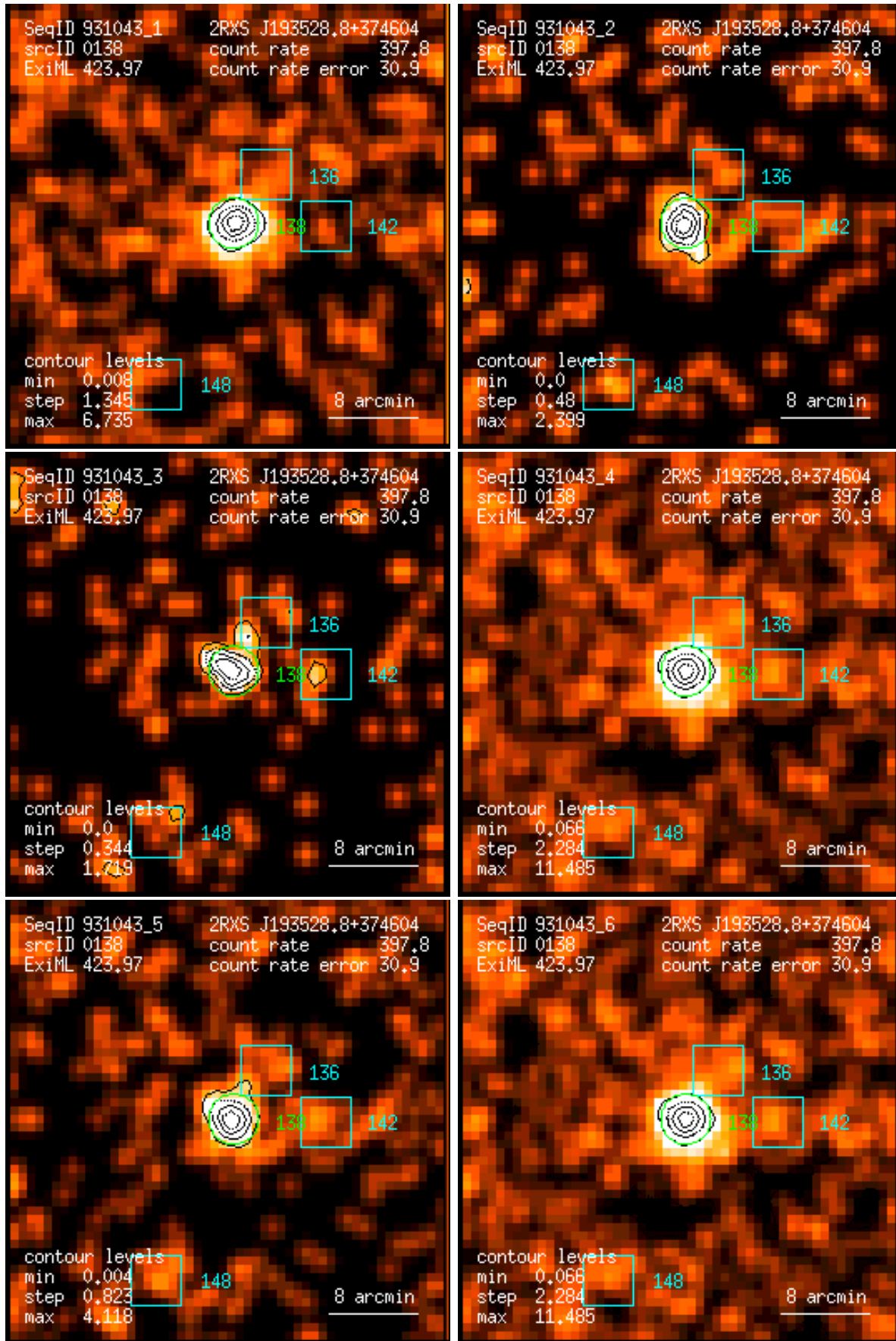
Figure 138: RASS 931043: detection 0138: band rate images, Gaussian filter: (1) PSPC channels 11 – 41, (2) 52 – 90, (3) 91 – 201, (4) 11 – 235, (5) 52 – 201, (6) 11 – 201. Broad band rates in counts/ks. Band rate contour levels in counts/ks/arcmin 2 .
