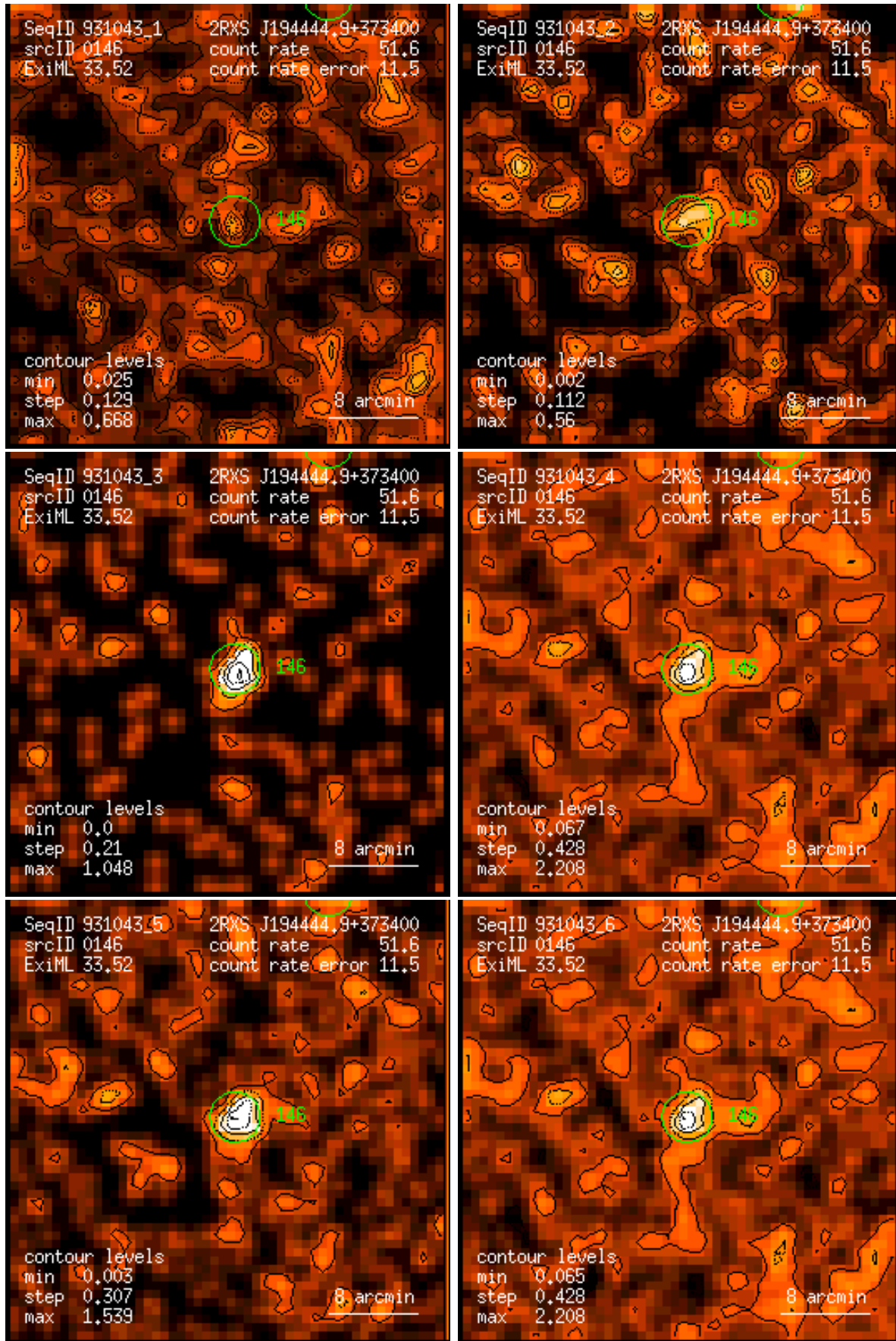
Figure 146: RASS 931043: detection 0146: band rate images, Gaussian filter: (1) PSPC channels 11 – 41, (2) 52 – 90, (3) 91 – 201, (4) 11 – 235, (5) 52 – 201, (6) 11 – 201. Broad band rates in counts/ks. Band rate contour levels in counts/ks/arcmin 2 .
