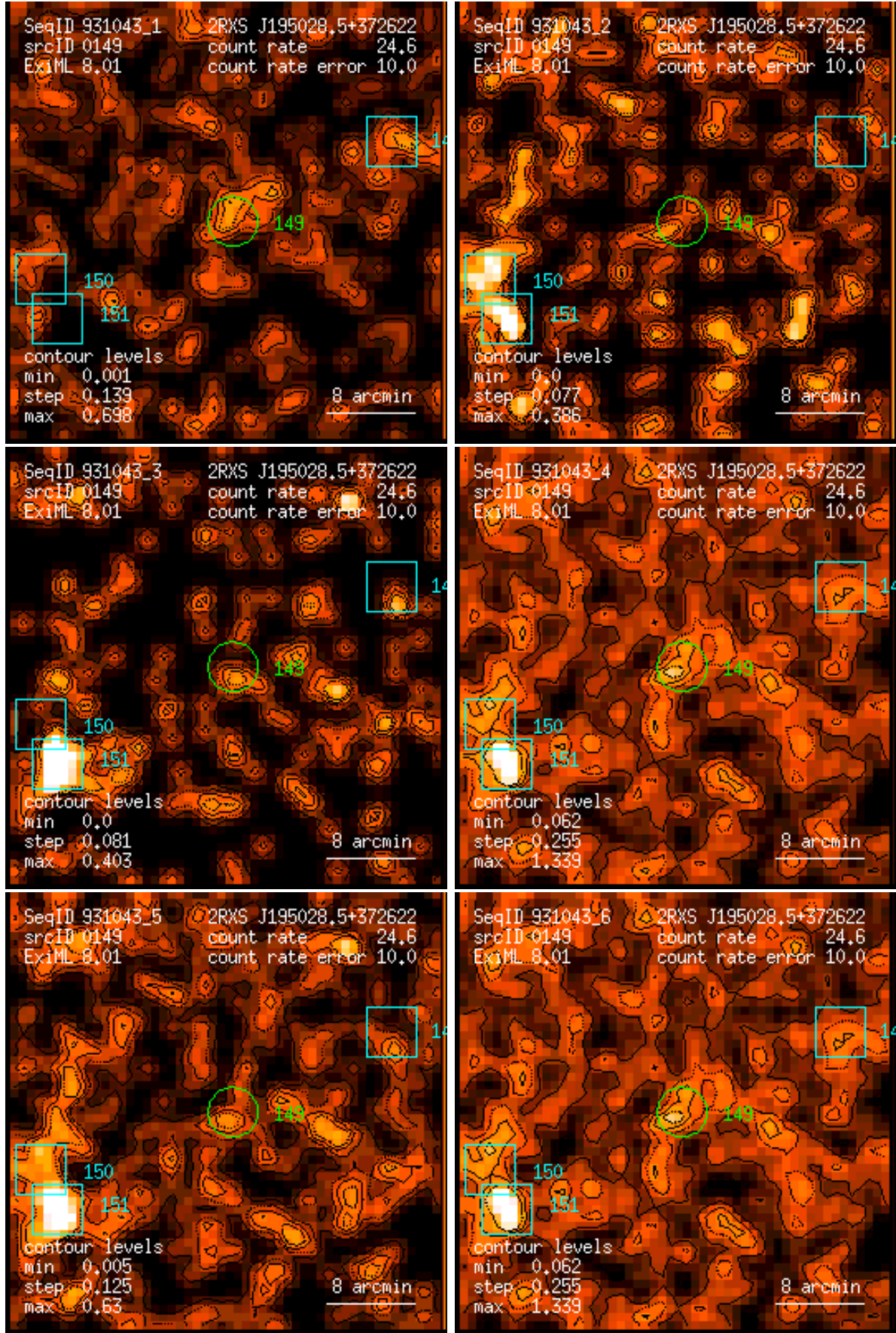
Figure 149: RASS 931043: detection 0149: band rate images, Gaussian filter: (1) PSPC channels 11 – 41, (2) 52 – 90, (3) 91 – 201, (4) 11 – 235, (5) 52 – 201, (6) 11 – 201. Broad band rates in counts/ks. Band rate contour levels in counts/ks/arcmin 2 .
