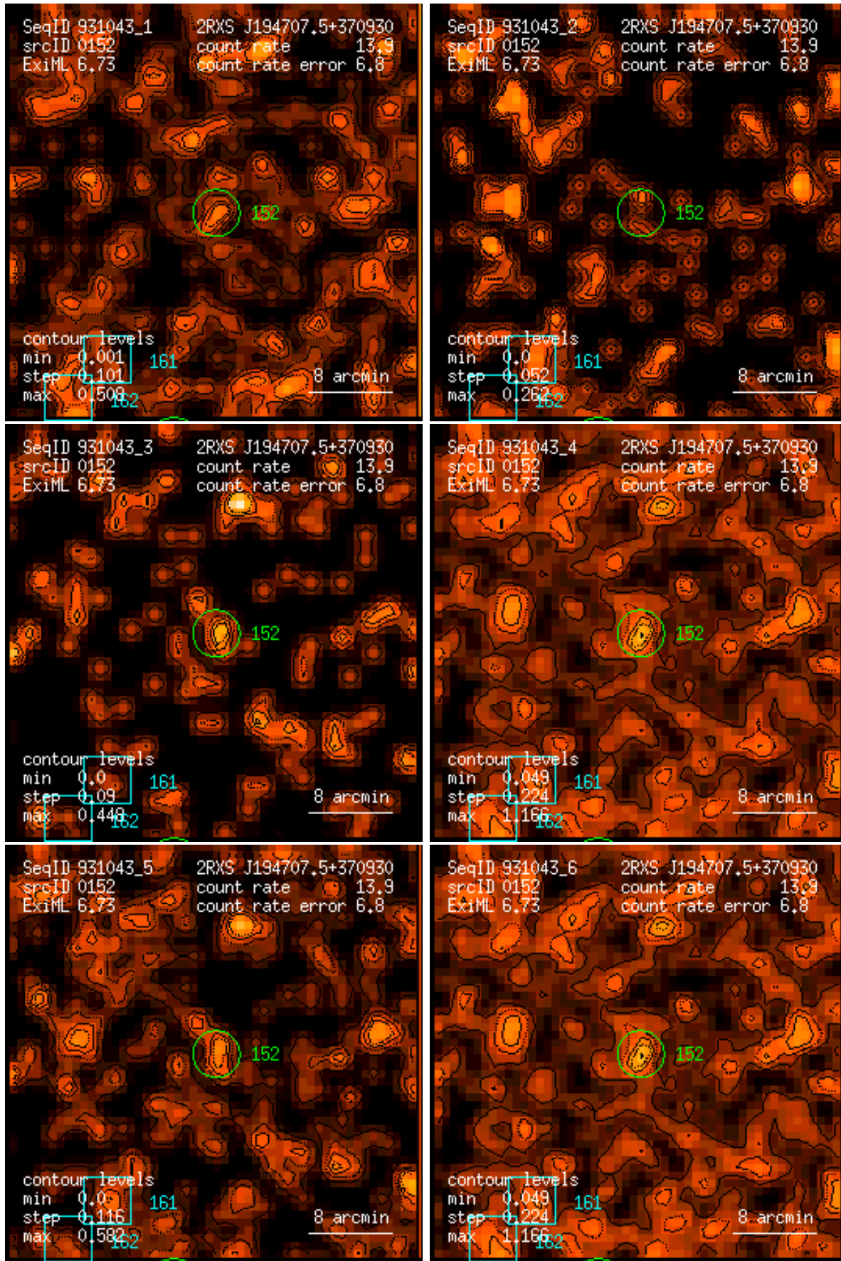
Figure 152: RASS 931043: detection 0152: band rate images, Gaussian filter: (1) PSPC channels 11 – 41, (2) 52 – 90, (3) 91 – 201, (4) 11 – 235, (5) 52 – 201, (6) 11 – 201. Broad band rates in counts/ks. Band rate contour levels in counts/ks/arcmin 2 .
