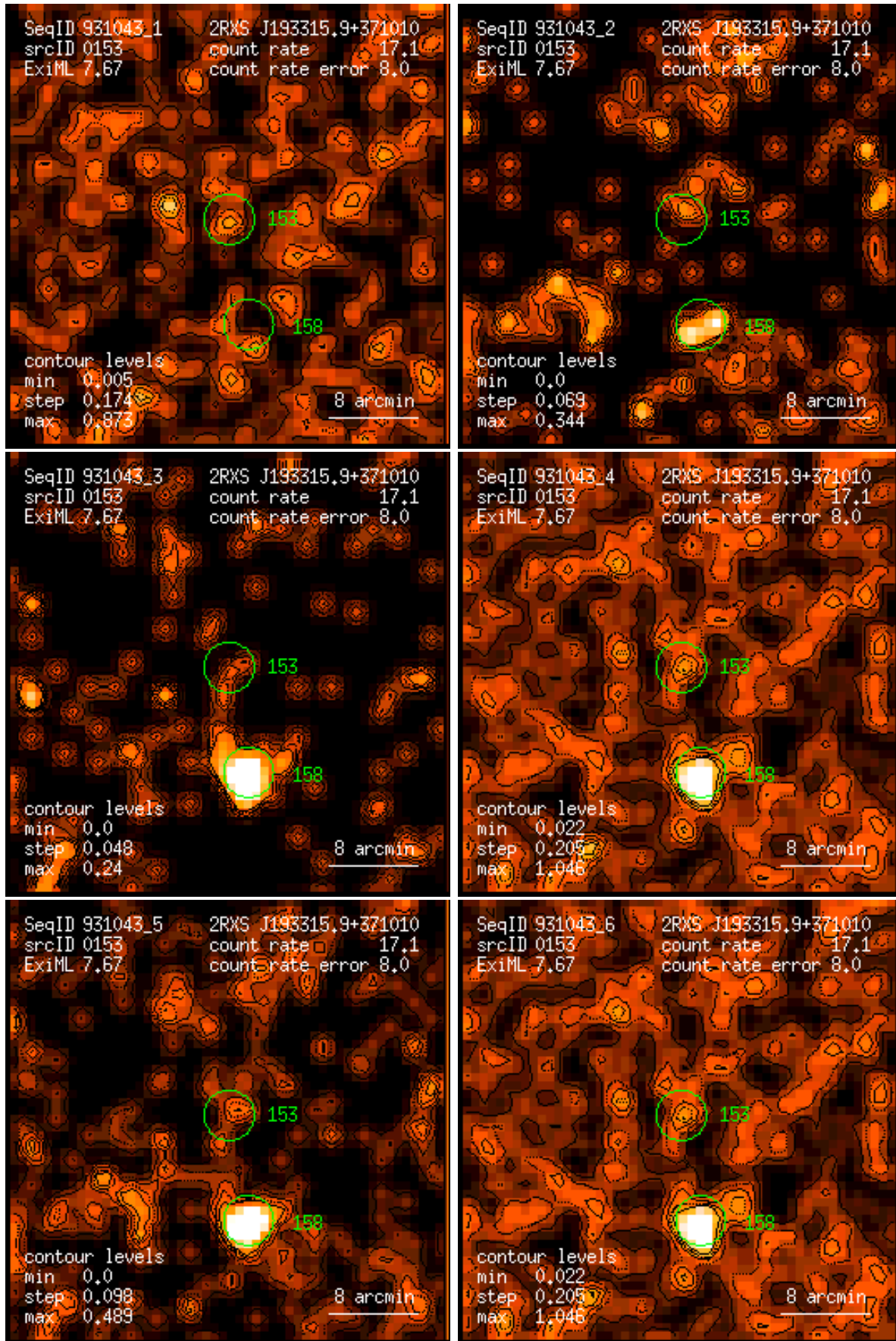
Figure 153: RASS 931043: detection 0153: band rate images, Gaussian filter: (1) PSPC channels 11 – 41, (2) 52 – 90, (3) 91 – 201, (4) 11 – 235, (5) 52 – 201, (6) 11 – 201. Broad band rates in counts/ks. Band rate contour levels in counts/ks/arcmin 2 .
