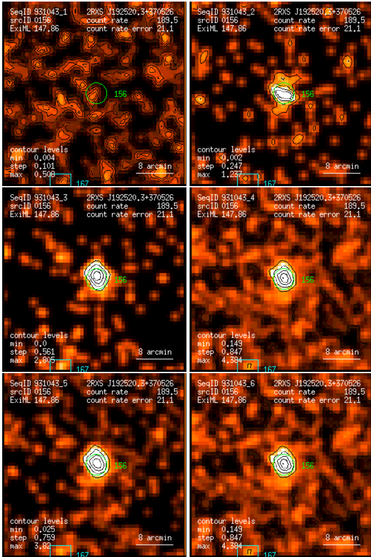
Figure 156: RASS 931043: detection 0156: band rate images, Gaussian filter: (1) PSPC channels 11 – 41, (2) 52 – 90, (3) 91 – 201, (4) 11 – 235, (5) 52 – 201, (6) 11 – 201. Broad band rates in counts/ks. Band rate contour levels in counts/ks/arcmin 2 .
