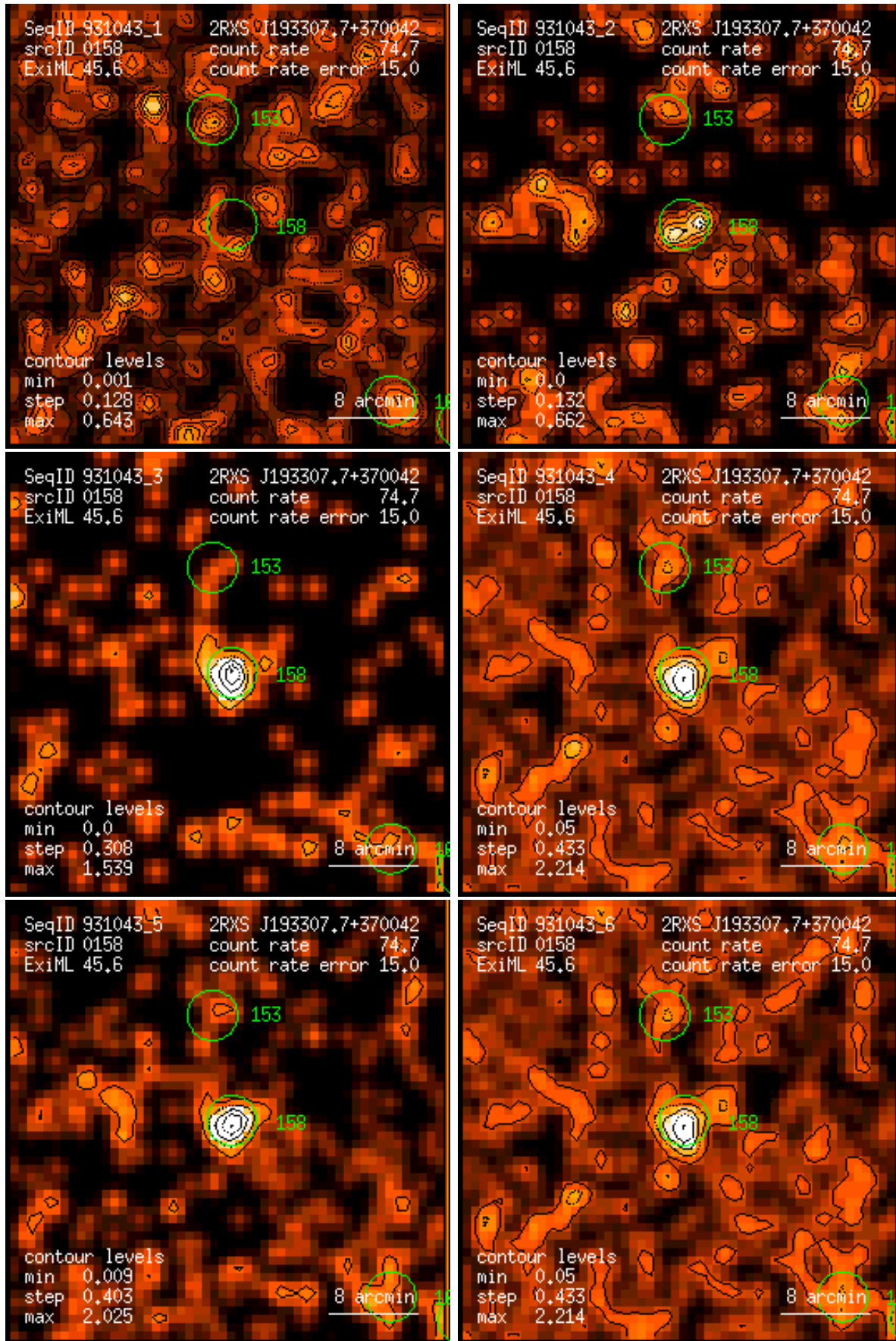
Figure 158: RASS 931043: detection 0158: band rate images, Gaussian filter: (1) PSPC channels 11 – 41, (2) 52 – 90, (3) 91 – 201, (4) 11 – 235, (5) 52 – 201, (6) 11 – 201. Broad band rates in counts/ks. Band rate contour levels in counts/ks/arcmin 2 .
