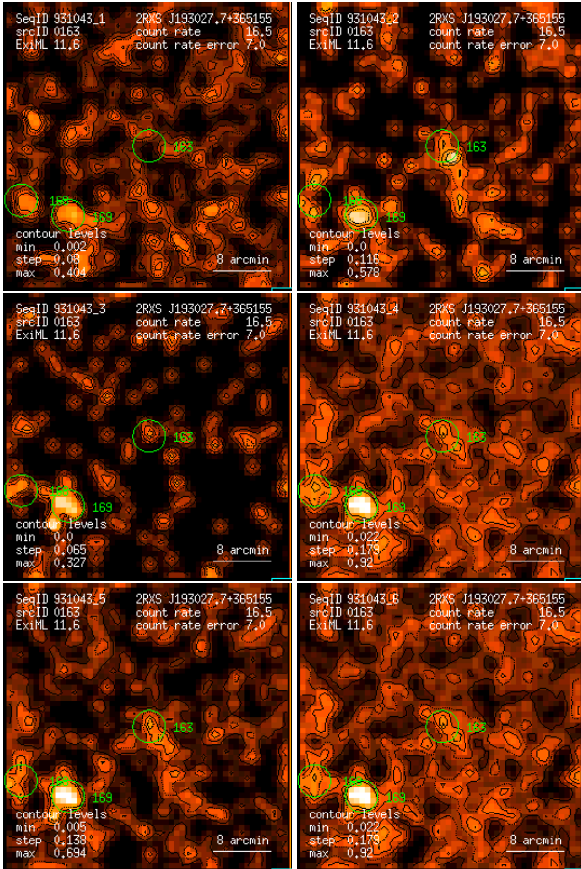
Figure 163: RASS 931043: detection 0163: band rate images, Gaussian filter: (1) PSPC channels 11 – 41, (2) 52 – 90, (3) 91 – 201, (4) 11 – 235, (5) 52 – 201, (6) 11 – 201. Broad band rates in counts/ks. Band rate contour levels in counts/ks/arcmin 2 .
