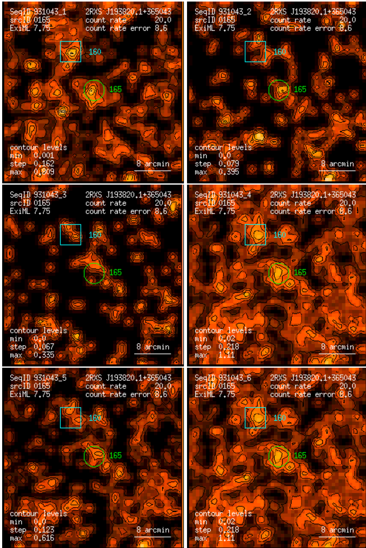
Figure 165: RASS 931043: detection 0165: band rate images, Gaussian filter: (1) PSPC channels 11 – 41, (2) 52 – 90, (3) 91 – 201, (4) 11 – 235, (5) 52 – 201, (6) 11 – 201. Broad band rates in counts/ks. Band rate contour levels in counts/ks/arcmin 2 .
