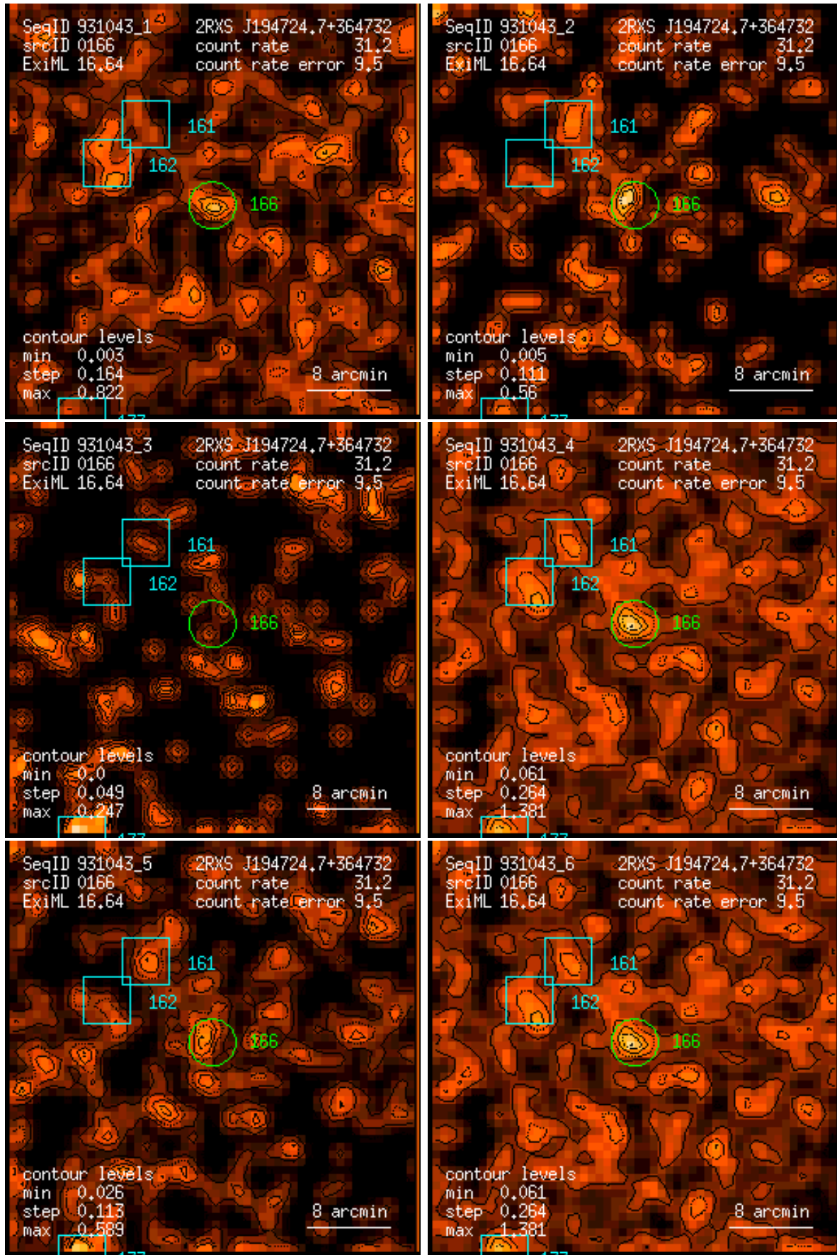
Figure 166: RASS 931043: detection 0166: band rate images, Gaussian filter: (1) PSPC channels 11 – 41, (2) 52 – 90, (3) 91 – 201, (4) 11 – 235, (5) 52 – 201, (6) 11 – 201. Broad band rates in counts/ks. Band rate contour levels in counts/ks/arcmin 2 .
