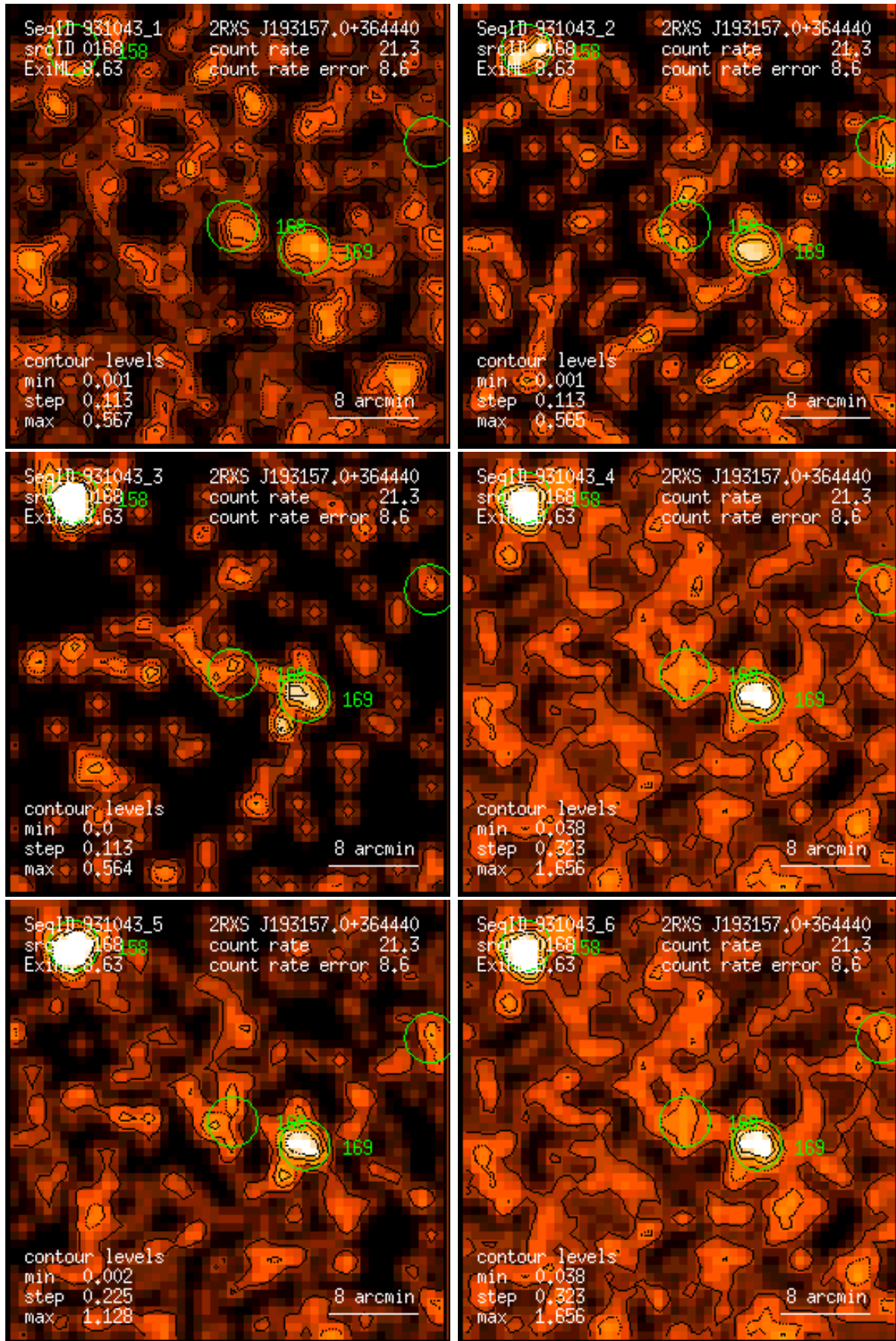
Figure 168: RASS 931043: detection 0168: band rate images, Gaussian filter: (1) PSPC channels 11 – 41, (2) 52 – 90, (3) 91 – 201, (4) 11 – 235, (5) 52 – 201, (6) 11 – 201. Broad band rates in counts/ks. Band rate contour levels in counts/ks/arcmin 2 .
