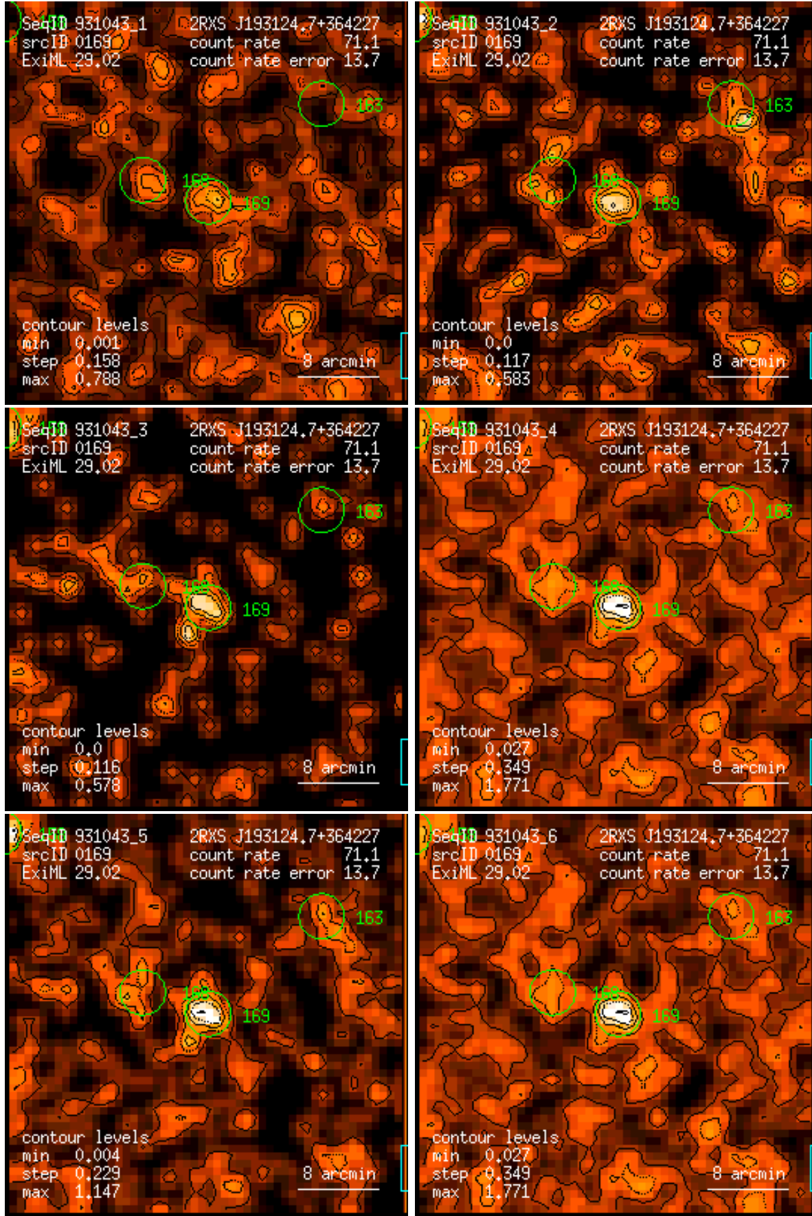
Figure 169: RASS 931043: detection 0169: band rate images, Gaussian filter: (1) PSPC channels 11 – 41, (2) 52 – 90, (3) 91 – 201, (4) 11 – 235, (5) 52 – 201, (6) 11 – 201. Broad band rates in counts/ks. Band rate contour levels in counts/ks/arcmin 2 .
