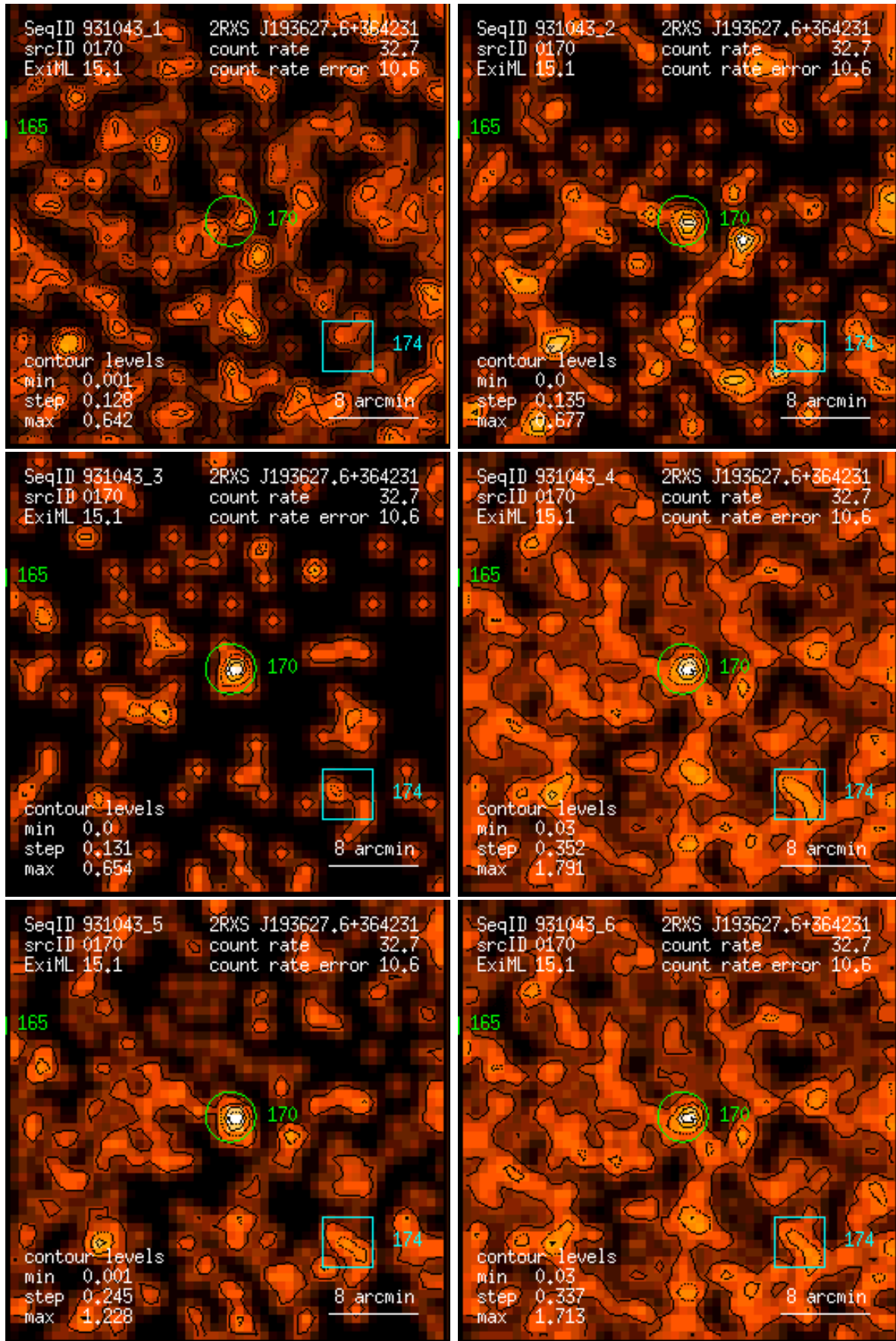
Figure 170: RASS 931043: detection 0170: band rate images, Gaussian filter: (1) PSPC channels 11 – 41, (2) 52 – 90, (3) 91 – 201, (4) 11 – 235, (5) 52 – 201, (6) 11 – 201. Broad band rates in counts/ks. Band rate contour levels in counts/ks/arcmin 2 .
